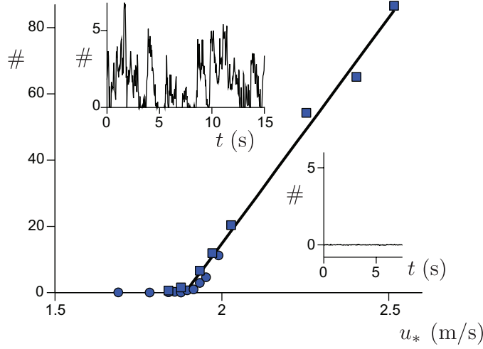
Figure 7: Equivalent of Fig. 3a, but at low pressure P = 10^3 Pa. Circles: data upon increasing the wind speed. Squares: data upon decreasing the wind speed. The solid line is the best linear fit through the data. Data dispersion provides an idea of the error made due to the finite observation time and the long relaxation time. Insets: typical signals above (left) and below (right) threshold.
