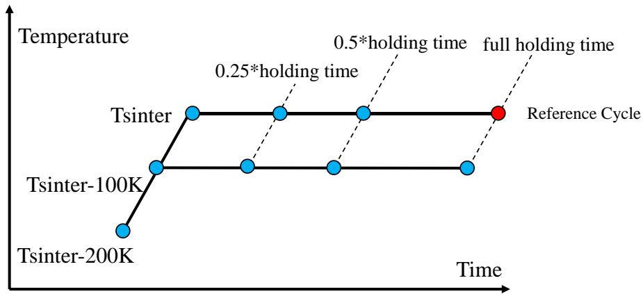
Figure 2 Schematic of interrupted cycles study, T_{sinter} \sim 1800^{\circ}\text{C}
