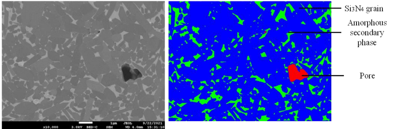
Figure 4 (Left) linear intercept on a \text{Si}_3\text{N}_4 polished surface sample micrograph at x10.000. (Right) colored micrograph for the calculation of phase proportions ( \text{Si}_3\text{N}_4 grains in blue, the amorphous secondary phase in green and pores in red)
