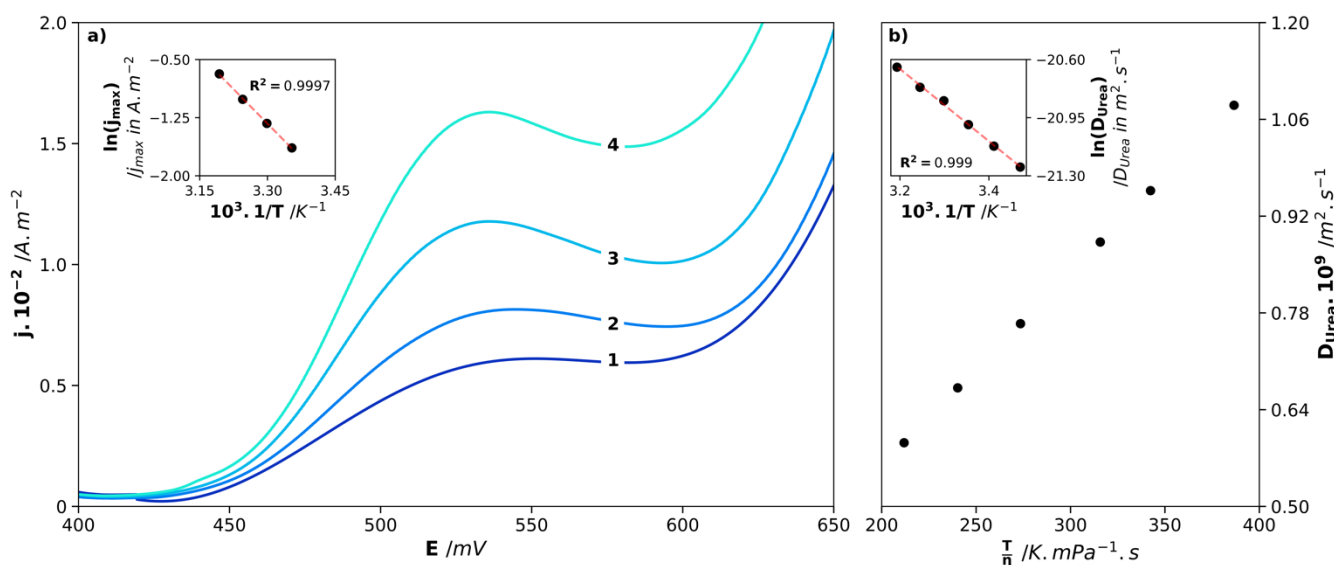
Fig. 9. a) Effect of temperature on the voltammograms obtained at 0.66 mV.s -1 , on nickel RDE in a 1 mol.L -1 KOH solution containing 0.33 mol.L -1 urea. The temperature used was 298 K (1), 303 K (2), 308 K (3) and 313 K (4). \omega = 200 RPM. Inset: \ln(j_{max}) = f(1/T) plotted to determine the activation energy of the global process.
