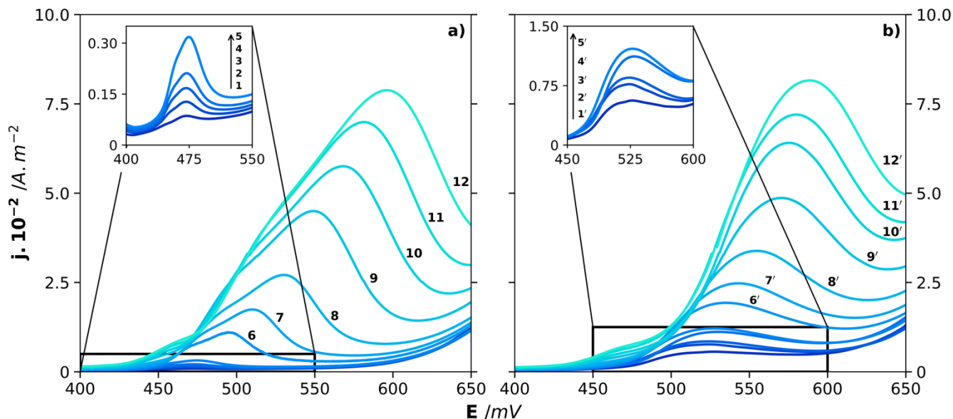
Fig. 4. Effect of potential scan rate on the voltammograms obtained without agitation on nickel electrode immersed into a) in 1 mol.L -1 KOH solution b) in 1 mol.L -1 KOH containing 0.05 mol.L -1 of urea. The scan rate used was 0.58 mV.s -1 (1-1'), 1.36 mV.s -1 (2-2'), 2.16 mV.s -1 (3-3'), 2.91 mV.s -1 (4-4'), 5 mV.s -1 (5-5'), 25 mV.s -1 (6-6'), 50 mV.s -1 (7-7'), 100 mV.s -1 (8-8'), 200 mV.s -1 (9-9'), 300 mV.s -1 (10-10'), 400 mV.s -1 (11-11') and 500 mV.s -1 (12-12'). The insets show a zoom in the oxidation peaks at low potential scan rate.
