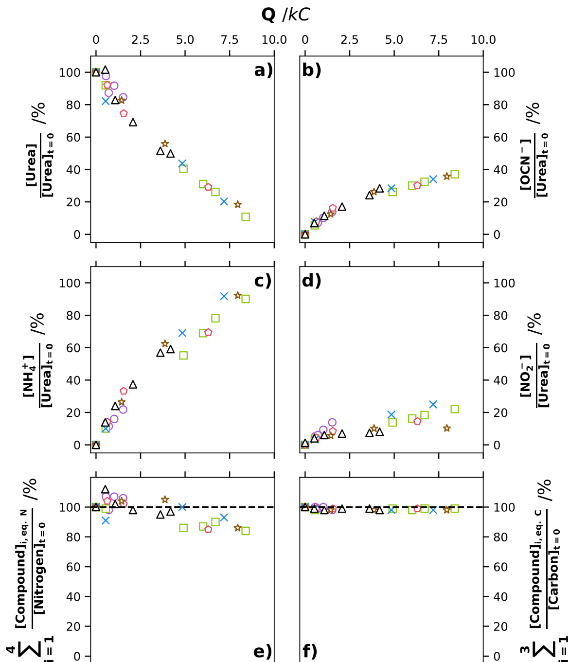
Fig. 13. Results of an indirect electrooxidation of urea in a stirred undivided cell (Metrohm type cell, represented by cell b) in Fig. 1) using various KOH concentration. E_{\text{applied}} = 550 \text{ mV} ; T = 298 \text{ K} ; [\text{CO}(\text{NH}_2)_2]_{t=0} = 0.33 \text{ mol.L}^{-1} ; S = 4 \text{ cm}^2 ; V = 50 \text{ mL} ; stirred by magnetic bar ( \omega = 500 \text{ RPM} , length of the bar: 2 cm; diameter of the bottom area of the cell: 4 cm). The results are presented as the evolution of the normalized concentration of the different byproducts as a function of the amount of supplied charge. Urea, cyanate, ammonium, and nitrite are shown in parts (a), (b), (c), and (d), respectively. The nitrogen mass balance, e), and carbon mass balance, f), are normalized with respect to the initial concentration. The KOH concentrations used are \circ 1, \square 1.5, \blacksquare 2.5, \times 3, \star 4, and \triangle 5 mol.L -1 . The uncertainties are smaller than 5.1%.
