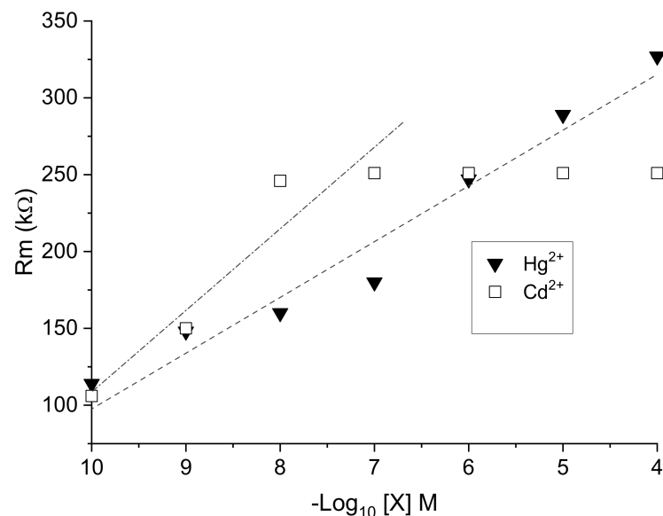
Figure 12. Variation in the membrane resistance R_m of EPS-functionalized electrochemical sensor as a function of -\log[\text{X}] for \text{X} = \text{Hg}^{2+} and \text{Cd}^{2+} .
