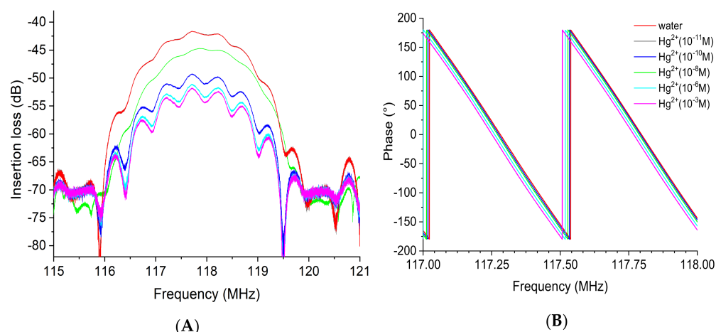
Figure 14. Superposition of the transmission response of the EPS-functionalized sensor with increasing mercury concentration from 10^{-11} to 10^{-3} M: (A) insertion loss or gain module and (B) phase. Both insertion losses (left) and phase (right) are plotted over a narrow frequency range centered on the acoustic resonance frequency.
