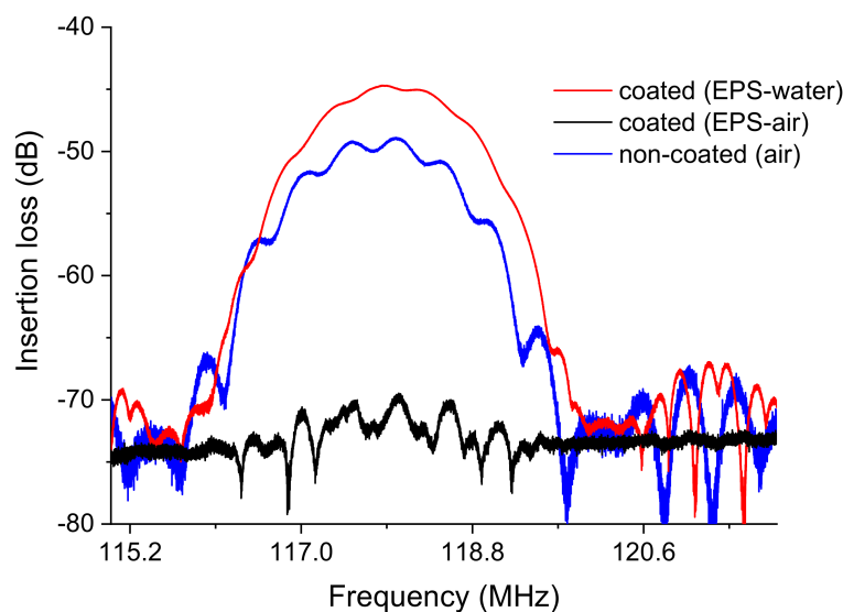
Figure 13. S21 transmission insertion losses of the Love wave sensor: noncoated with Graesiella sp. EPS in air and coated with Graesiella sp. EPS in air and water measured with VNA (vector network analyzer).
