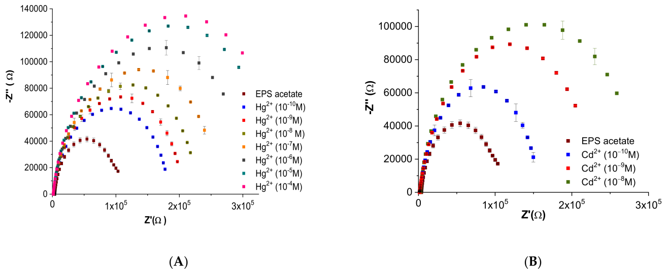
Figure 11. Nyquist plots of the gold electrodes coated with EPS membrane in acetate ( 10^{-2} M, pH 6.8) for a series of different concentrations of (A) mercury ( Hg^{2+} ) and (B) cadmium ( Cd^{2+} ) (values are presented as the mean of triplicate measurements ( n = 3 ; \pm SD)).
