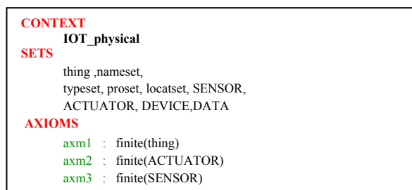
Fig.5. An Event-B model for IoT Architecture: the context (1)
