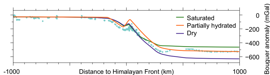
FIGURE 6 Gravimetric control on the initial hydration level of the modelled Indian lower crust. Bouguer anomalies must first fit the far-field difference between the left and right ends of the profile before adjusting inner parts of the model. The large misfit between observed data (blue dots) as well as the dry and saturated composition models precludes the further use of these two models. The partially hydrated lower crustal composition model fits the far-field difference in gravity anomaly, and is further refined to fit the observed data in the central portion of the profile [Colour figure can be viewed at wileyonlinelibrary.com ]
