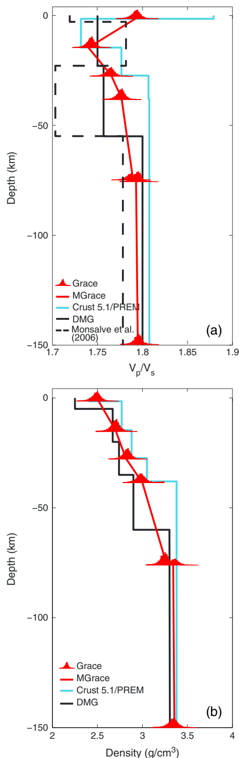
Figure 8. Comparison of 1-D models for P wave/S wave (a) velocities ratio and (b) density of the upper 150 km of the Earth: Crust 5.1/PREM (blue), regional models (solid black from Pandey et al. [1995], dashed black from Monsalve et al. [2006]), Grace (red histograms represent marginal posterior probability density functions), and MGrace, median derived from Grace.
