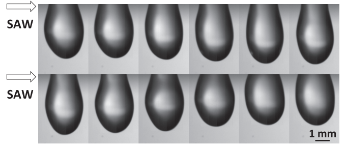
FIG. 6. Sequence of images (time elapsed between successive images: 4 ms, captured at 250 fps) of a drop of volume 15 \mu l ( Bo = 0.5 ) excited with an acoustic power corresponding to We_{ac} = 0.38 . The drop reaches a stable regime with large deformation but almost no oscillation and translation.
