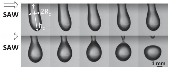
FIG. 7. Sequence of images (time elapsed between successive images: 2 ms, captured at 500 fps) showing the detachment of a drop of 10 \mu l excited with an acoustic power corresponding to We_{ac} = 0.41 . The parameters h_c and R_c are, respectively, the critical height and radius of the liquid column before breakup occurs.
