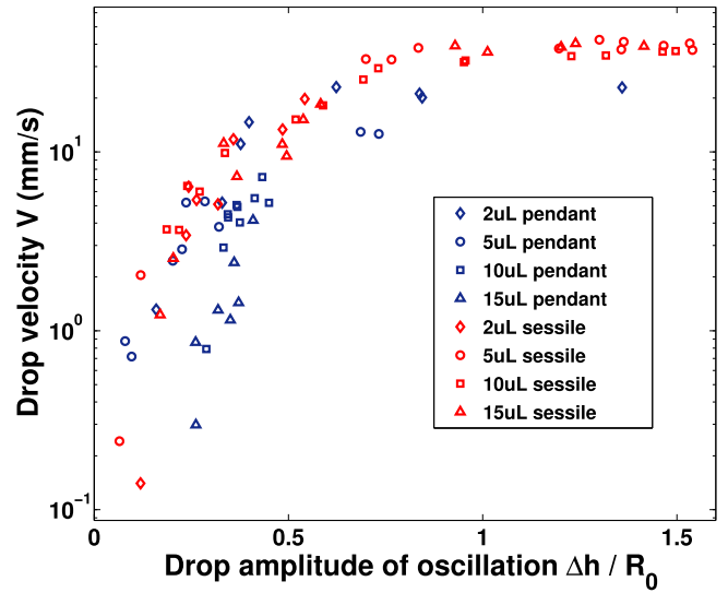
FIG. 13. Sessile (red or gray) and pendant (blue or black) drops translation speed as a function of the dimensionless amplitude \Delta h / R_o . The droplet velocity is measured from the side views of the drop motion by monitoring the position of the contact line and applying a low pass filter to suppress the effect of the drop oscillations.
