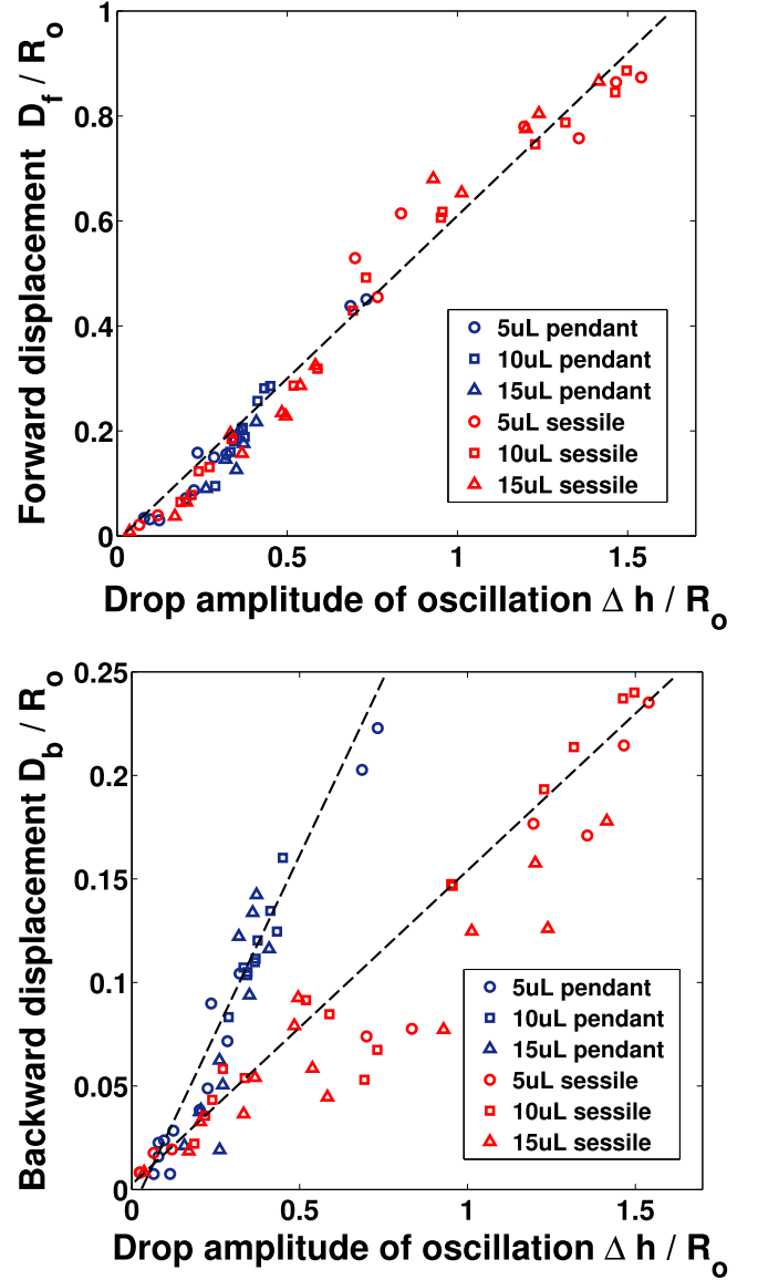
FIG. 15. Forward (up) and backward (down) displacement of the front part of the contact line of sessile (red or gray) and pendant (blue or dark) drops as a function of the dimensionless amplitude of oscillation \Delta h/R_o . The backward and forward displacements per cycle are calculated by monitoring the extreme positions of the contact line over one oscillation cycle, subtracting them to obtain the forward and backward displacements and averaging them over all the cycles in the stable regime.
