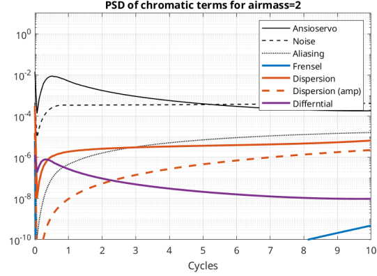
Figure 7. AO PSDs profiles for the different term in the AO error budget for a 50x50, 4kHz system under good seeing and airmass=2. We consider the worst case with \lambda_{SCI}=620\text{nm} and \lambda_{WFS}=1400\text{nm} .
