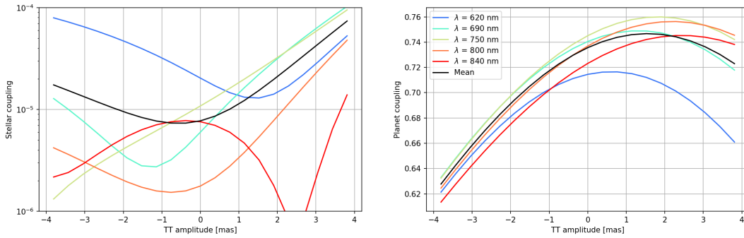
Figure 4. Tip-tilt sensitivity for a spider-free VLT aperture. Negative tilt pushes the star further away from the lenslet.
