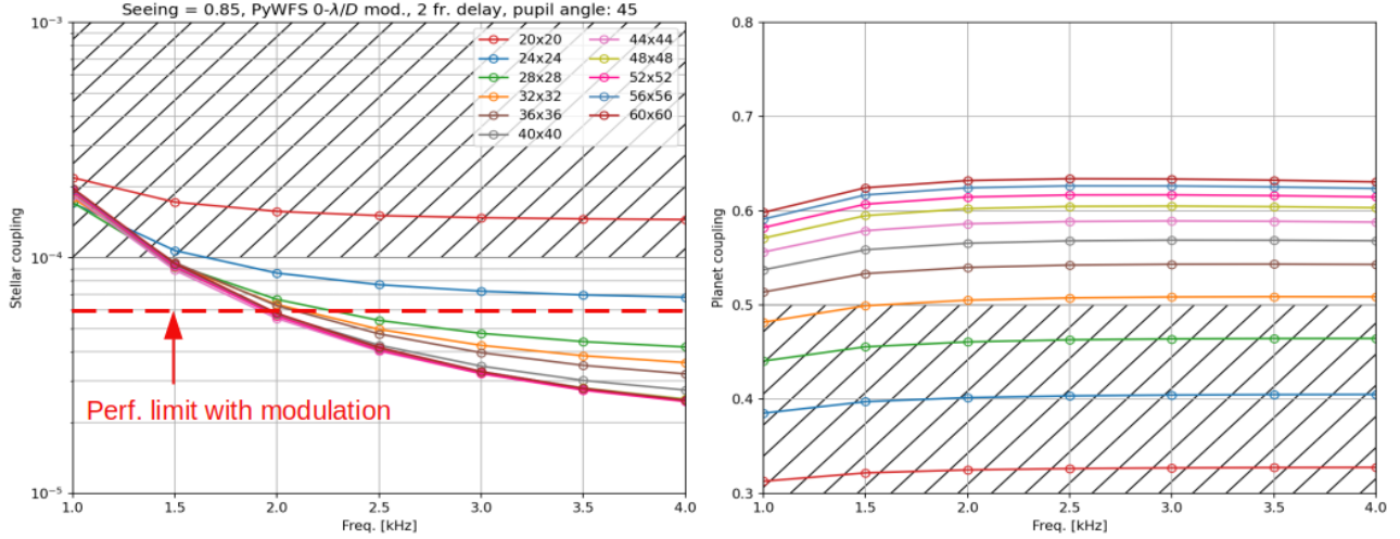
Figure 8. End-to-end RISTRETTO performance on Prox Cen as a function of loop speed. We consider a VLT pupil with spiders oriented to show an average behavior. On the left, the red dotted line shows the performance limit with modulation of 3\lambda/D .
