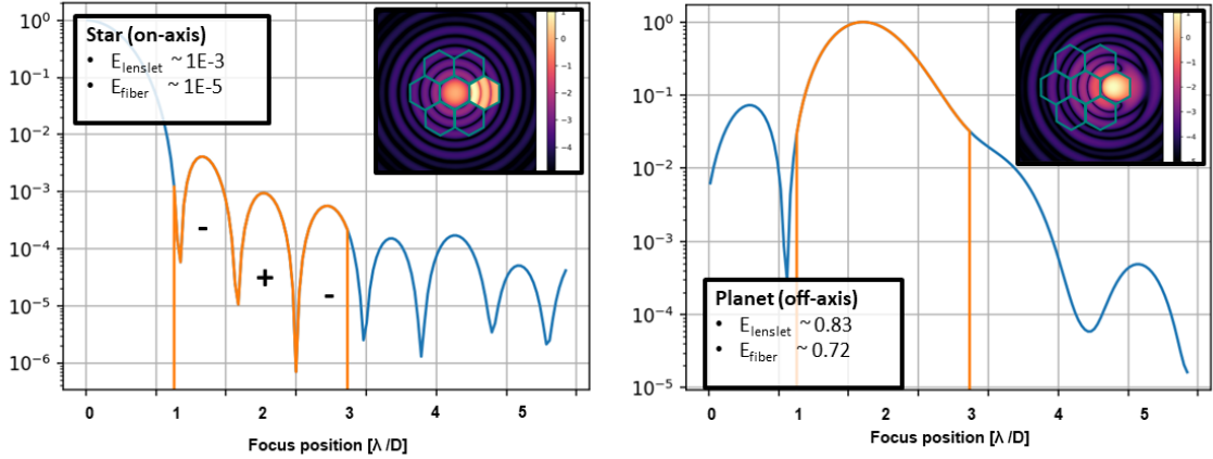
Figure 2. Example of post-PIAA PSF at \lambda = 750 nm. Left: on-axis (stellar) PSF: rings are attenuated by a factor \geq 10 compared to standard pupil and increase in frequency, providing some nulling level across a lenslet. Right: off-axis (planet at 2\lambda/D ) PSF with moderate aberrations.
