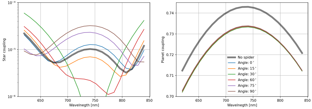
Figure 3. Stellar and planet coupling as a function of wavelength for a CaF2 PIAA. We show the case of VLT pupil (16.2% obstruction) without and with spiders, under different orientations with respect to the lenslet.
