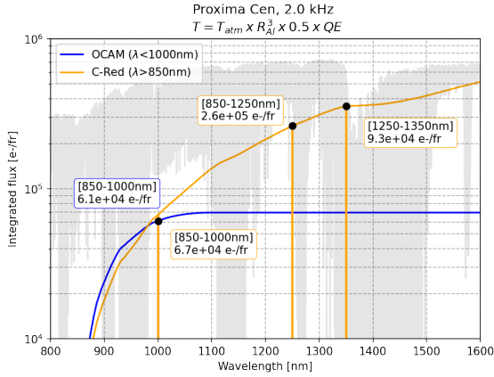
Figure 6. Photon budget on Prox Cen for 2kHz system.
