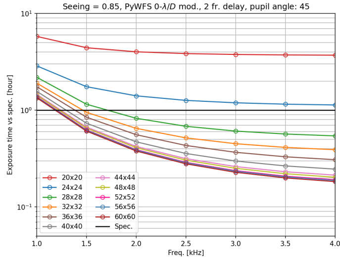
Figure 9. Potential gain in exposure time with respect to the requirement for the different AO configurations.
