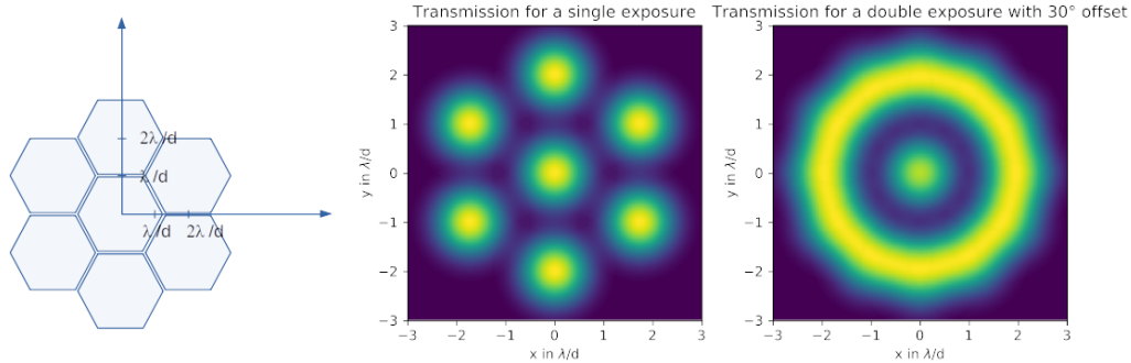
Figure 1. Left: schematic view of the RISTRETTO IFU. Middle: transmission map due to single mode fiber coupling. Right: transmission map after 30° rotation of the IFU.
