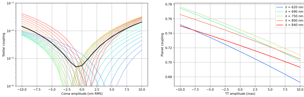
Figure 5. Sensitivity to coma aberration for a spider-free VLT aperture. Coloring on the left plot follows the logic of the right plot, with finer wavelength sampling. Black curve on the left is the average over the band.
