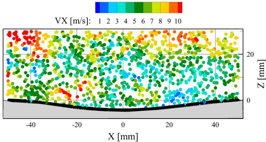
Figure 8 – Ground truth particles and markers of one of the HOMER internal datasets ( 2 mm thick slice in the Y direction). The moving lower wall is considered as an aluminum panel of 0.5 mm thickness, actuated with a periodic vertical forcing motion at its centre (defining the origin (\mathbf{X}, \mathbf{Z}) = (\mathbf{0}, \mathbf{0}) ). Particles are color-coded by their streamwise velocity and panel markers appear in black. From Sciacchitano et al. (2022).
