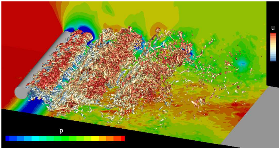
Figure 2 - Sample flow snapshot, including Q-criterion iso-surfaces color-coded by streamwise velocity u , iso-contours of pressure p at the lower and side walls.
