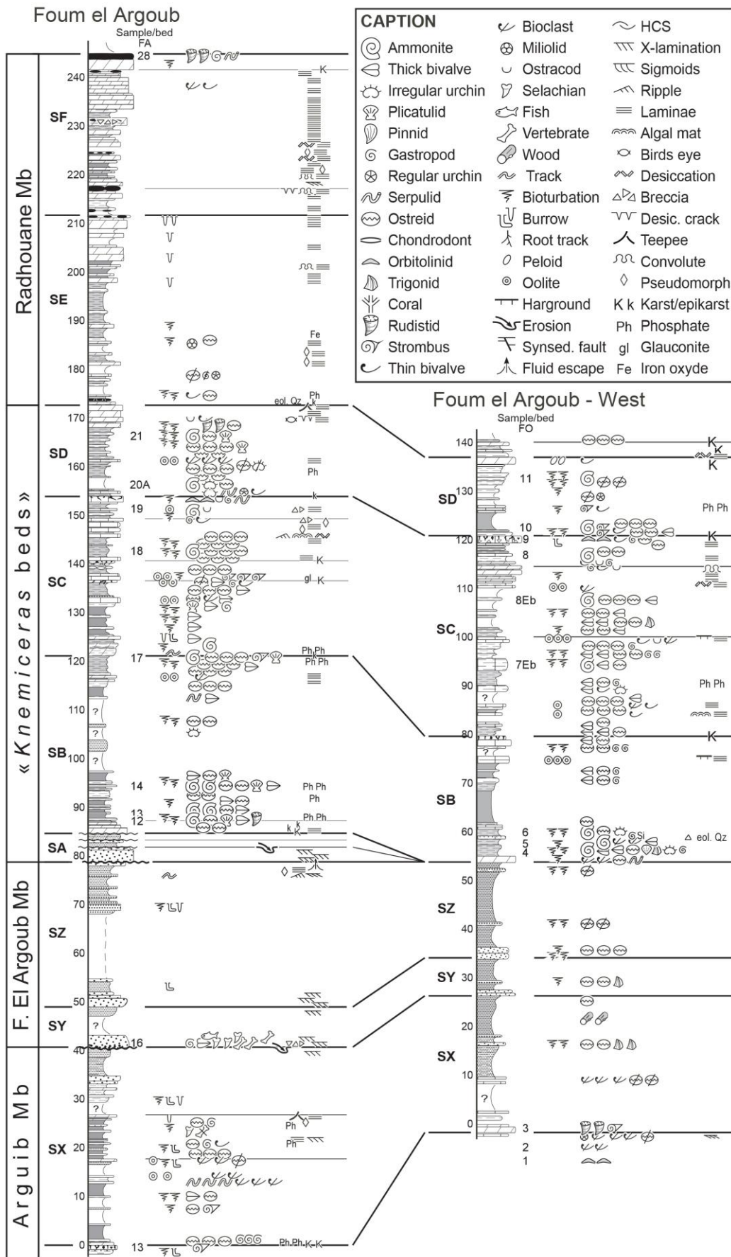
Figure 6. Lithology and sedimentology of the Foum el Argoub sections.
