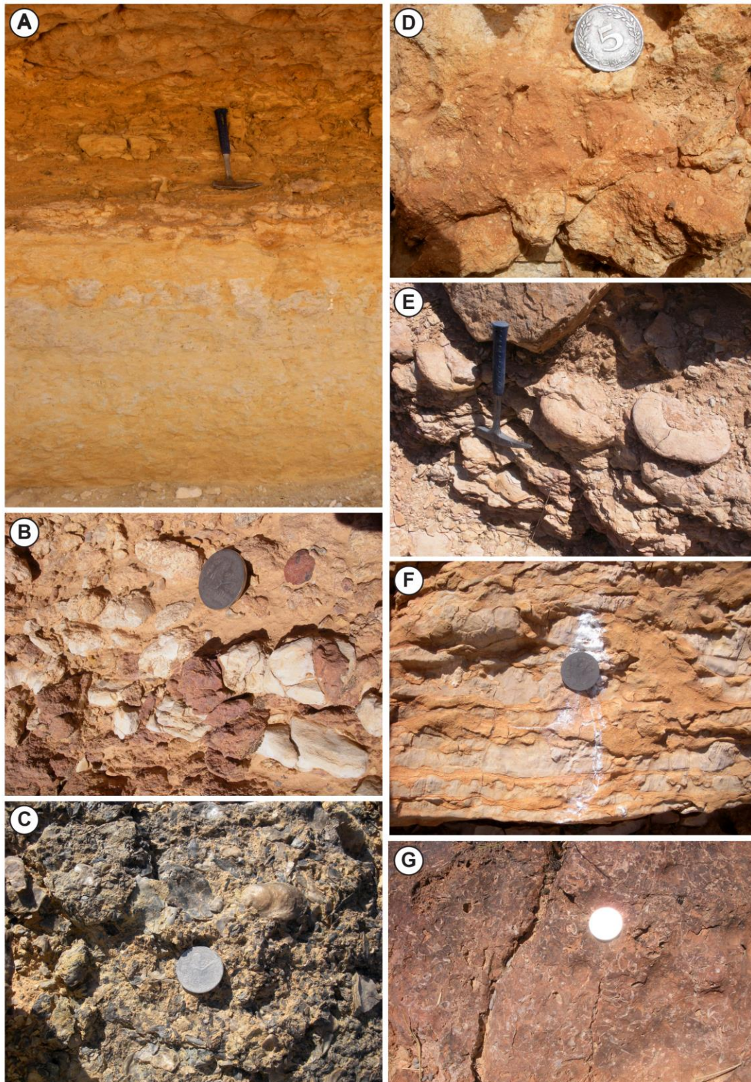
Figure 7. Aspects of the sedimentation of the “Knemiceras beds” and Radhouane Member. (A) Alteration and pedogenesis below the massive orbitolinid-rich limestone bed (top SZ) (Foum el Argoub section, m 78). (B) Intense karstification, interpreted as a sequence boundary (Bir Oum Ali North section, m 128 (top SB)). (C) Oyster coquina (Bir Oum Ali North section, m 145 (SC)). (D) Karstified, orbitolinid-rich limestone, interpreted as a sequence boundary (Bir Oum Ali North section, m 164 (top SC)). (E) Layer rich in Parengonoceras bussoni (Foum el Argoub West section, m 117 (SC)). (F) Laminated dolomitic limestone with tidal laminations (Foum el Argoub section, m 183 (SE)). (G) Silicified dolostone bearing numerous rudists (Foum el Argoub section, m 246 (top SF)).
