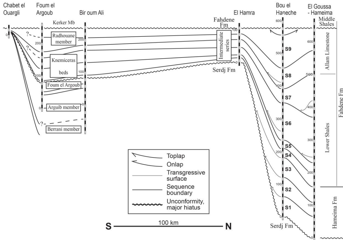
Figure 11. Correlation of the Chotts area with Central Tunisia sections. (above) Chronostratigraphic correlations; (below) Correlation of sequences and sedimentary units.
