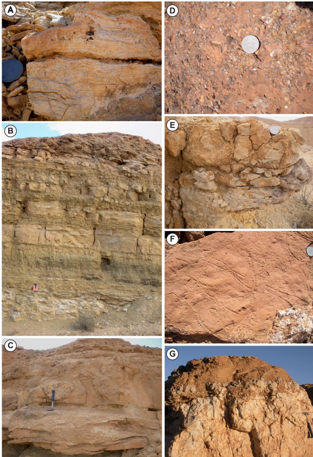
Figure 5. Aspects of the sedimentation of the Arguib and Foum el Argoub members. (A) Teepee structure in a thin calcareous bed at the base of the evaporite unit (Bir Oum Ali South section, m 1 (SX)). (B) Evaporites alternating with marls and thin limestone beds (Bir Oum Ali South section, m 8-15 (SX)). (C) Channel at the base of the Foum el Argoub Member (Bir Oum Ali South section, m 36 (base SY)). (D) Microconglomerate in a channel of the Foum el Argoub Member (Foum el Argoub section, m 43 (base SY)). (E) Limestone bed rich in nerineids, deeply karstified (Bir Oum Ali South section, m 49 (S2)). (F) Arthropod trackways near the top of the Foum el Argoub Member (Foum el Argoub section, m 77 (SZ)). (G) Top of the massive orbitolinid-rich limestone (Bir Oum Ali South section, m 78 (SA)).
