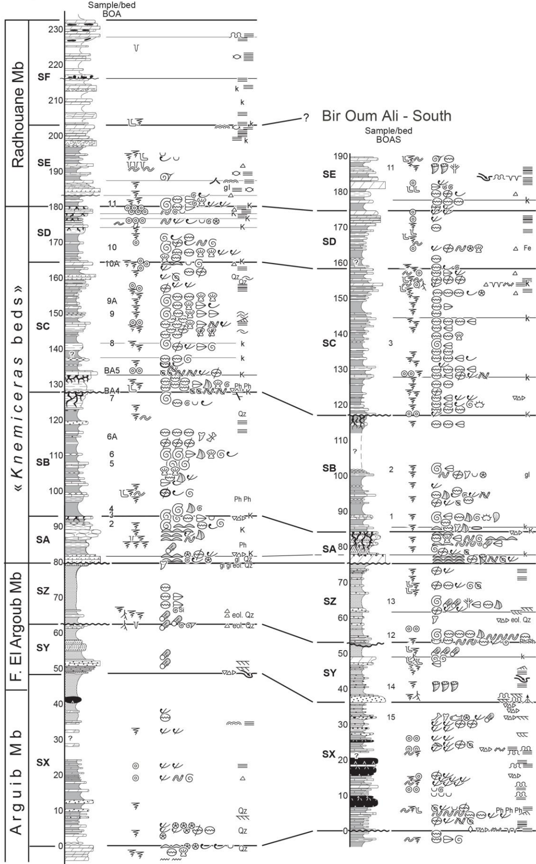
Figure 4. Lithology and sedimentology of the Bir Oum Ali sections. Caption on Figure 6.
