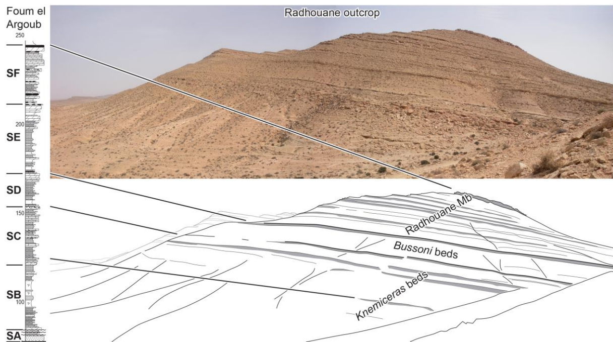
Figure 8. Radhouane outcrop, and correlations with the Foum el Argoub section.
