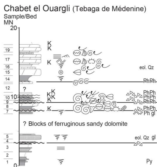
Figure 9. Lithology and sedimentology of the Chabet el Ouargli section.
