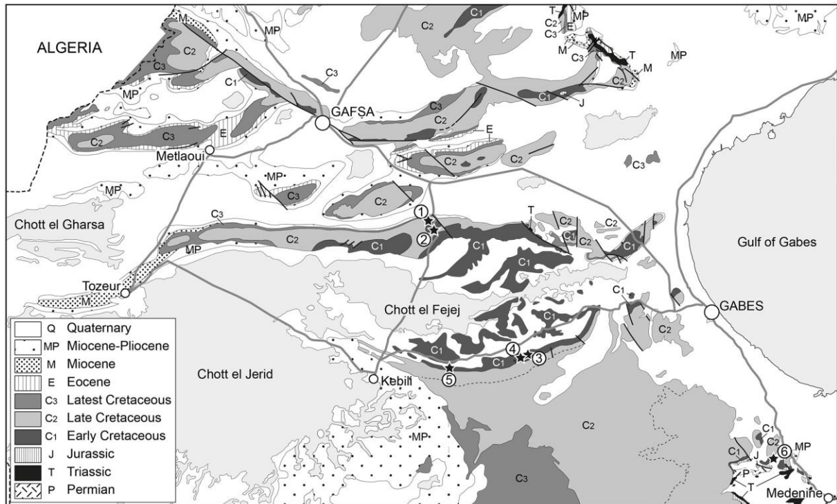
Figure 2. Geological map of the Chott area, showing the studied sections (location on Fig. 1). 1. Bir Oum Ali North, 2. Bir Oum Ali South, 3. Foum el Argoub, 4. Foum el Argoub West, 5. Radhouane.
