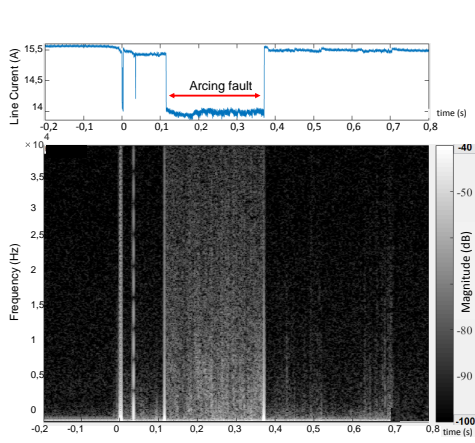
Figure 3: Spectrogram of a single resistive load powered by a 270 VDC source (opening electrodes test).
