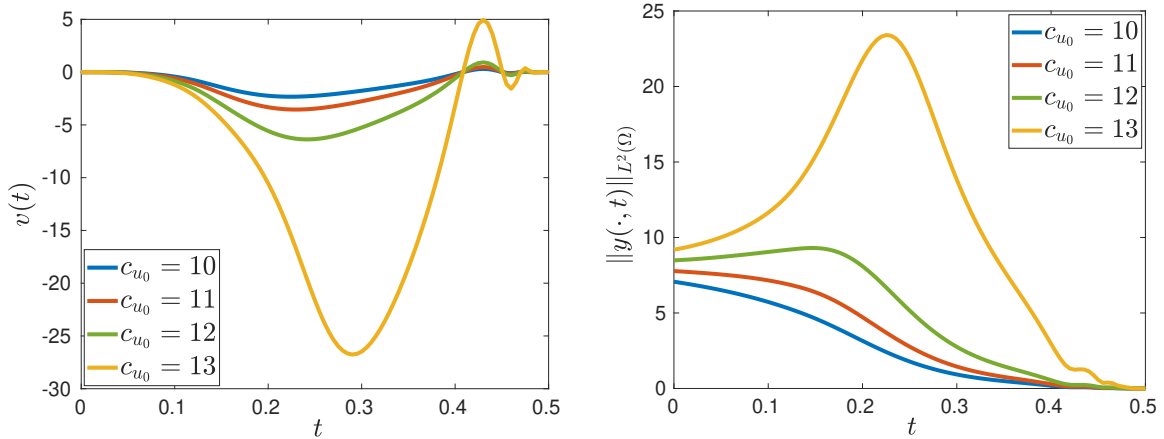
Figure 12: s = 3 ; f(r) = -r^2 ; u_0(x) = c_{u_0} \sin(\pi x) ; Left: Control functions v_{k^*} and Right: Evolution of \|y_{k^*}(\cdot, t)\|_{L^2(\Omega)} w.r.t. time t for different values of c_{u_0} .
