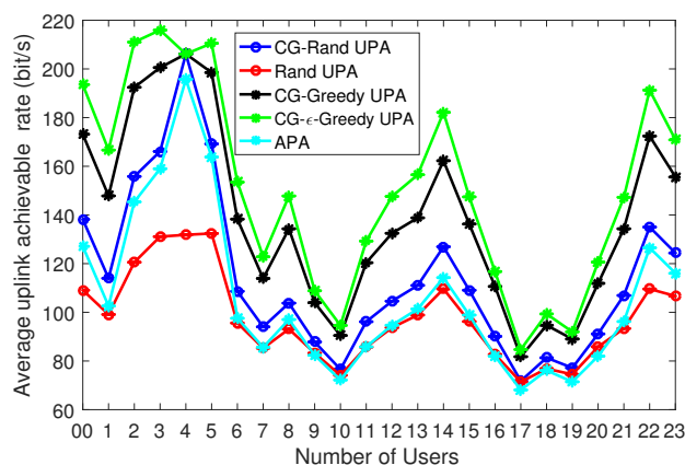
FIGURE 7. Average users uplink achievable rate
