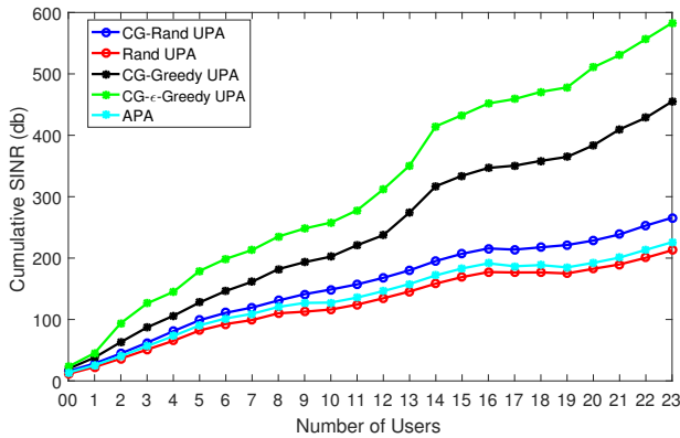
FIGURE 8. Cumulative SINR
