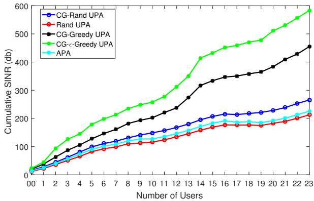
FIGURE 8. Cumulative SINR
