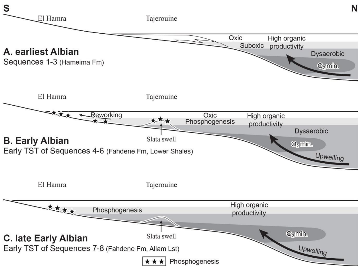
Fig. 13. Model for the evolution of the Tunisian margin during the Early Albian transgression, explaining the genesis of phosphate-rich and organic-rich deposits.
