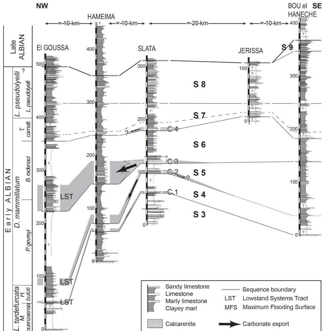
Fig. 7. Correlations of the sections studied in the Tajerouine area.
