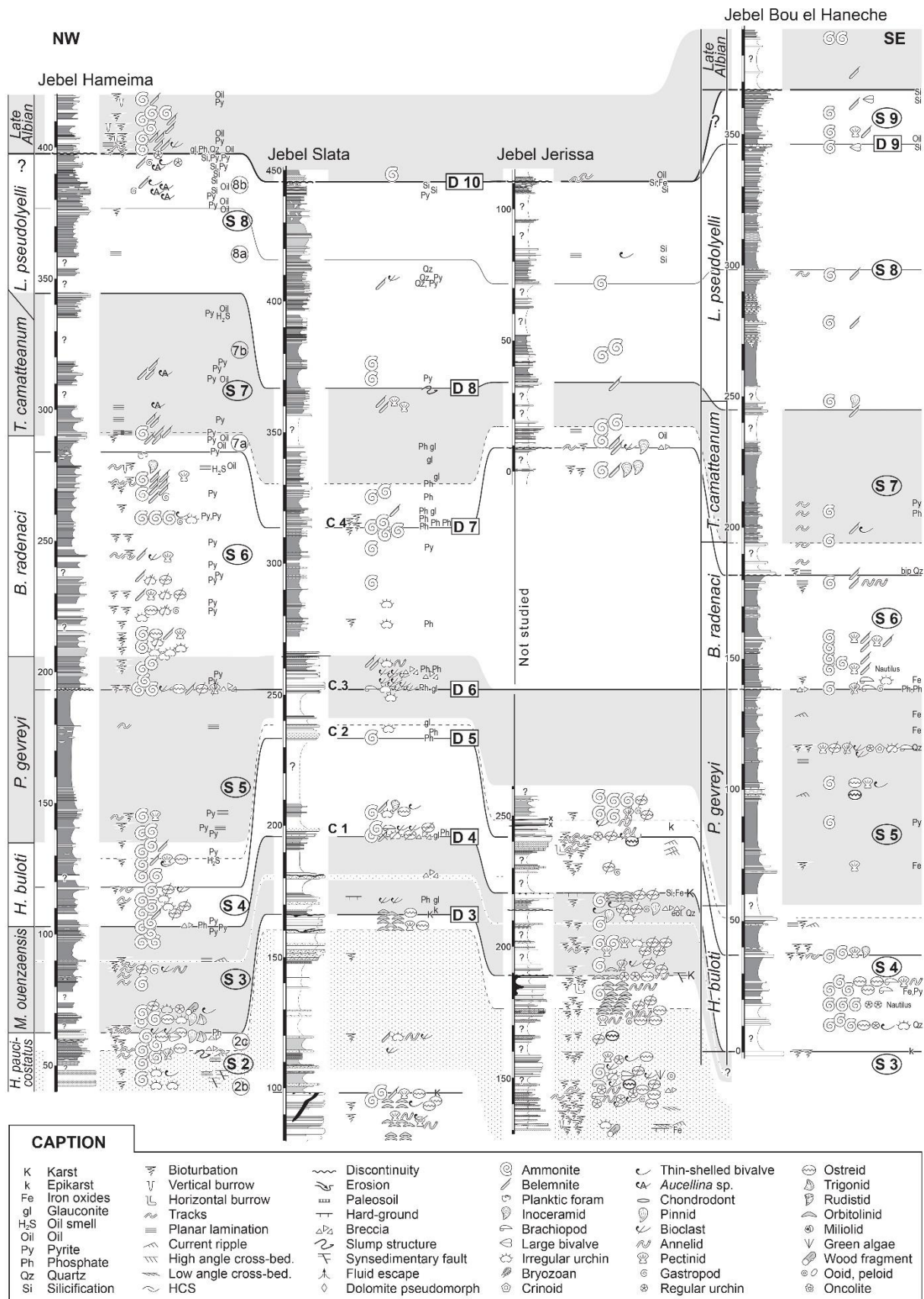
Fig. 5. Sections of the Fahdene Formation in the Tajerouine area: lithology, sedimentary features and correlations. Shaded areas: ammonite zones; Dotted area: Sandy unit of S2. Location on Fig. 3.
