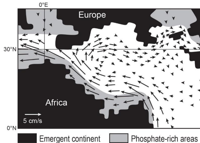
Fig. 12. Oceanic circulation in the Western Tethys, from Pohl et al. (2019), simplified.
