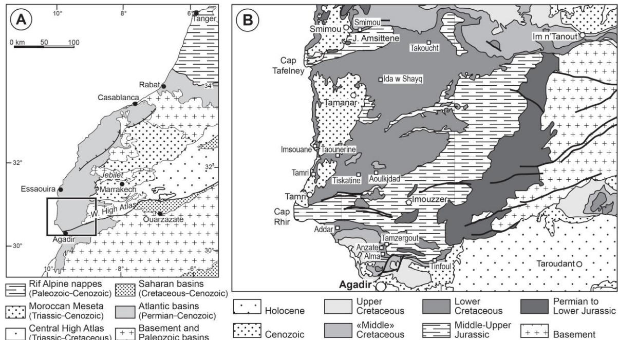
Figure 1. Location of the study area. A. Location of the Essaouira-Agadir basin. B. Geological sketch of the EAB, and location of the studied sections.
