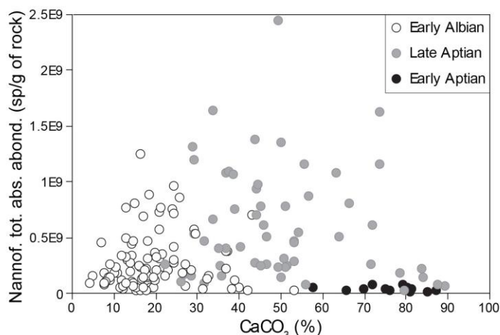
Figure 11. Bivariate plot showing the relationship between \text{CaCO}_3 content and calcareous nannofossil absolute abundance for different time intervals, recognized in the Essaouira-Agadir basin. 176 measurements from the Addar, Alma, Anzate, Ida w Shayq, Tinfoul and Tiskatine sections.
