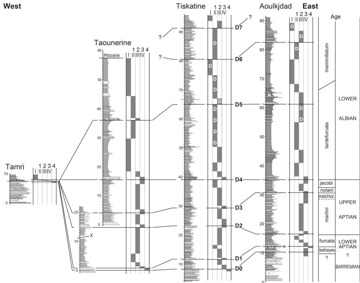
Figure 9. East-West correlations of the Aptian–lower Albian sections in the central part of the Essaouira-Agadir Basin. D: dysaerobic facies. See Fig. 10 for caption, and Fig. 3 for explanation of 1 to 4, and I to IV.
