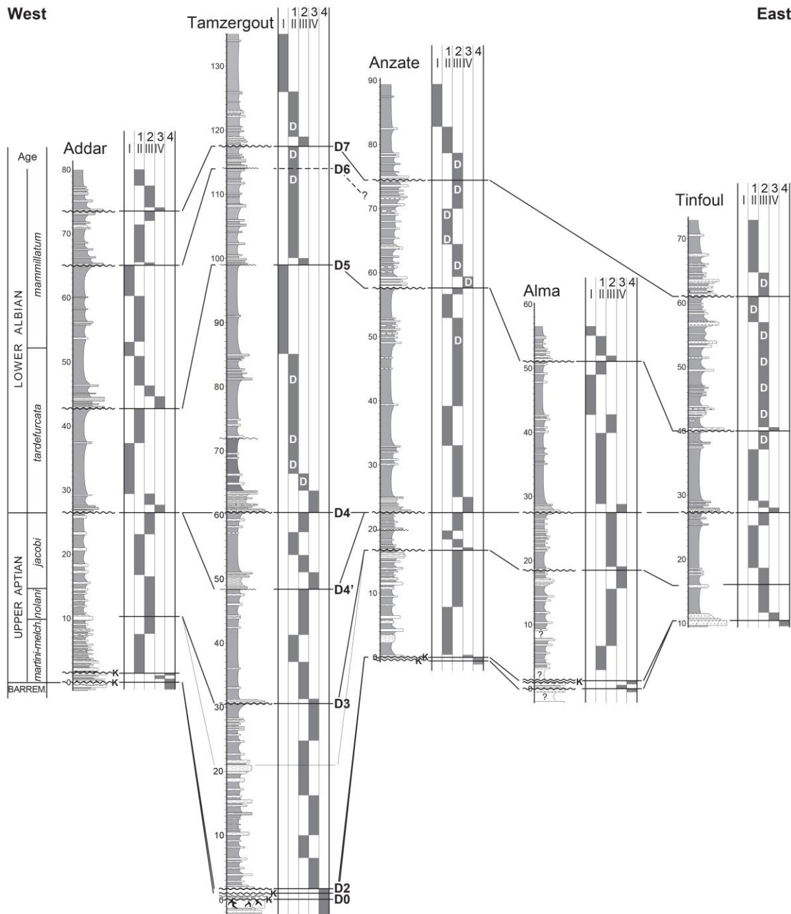
Figure 8. East-West correlations of the Aptian–lower Albian sections in the southern part of the Essaouira-Agadir basin. D: dysaerobic facies. See Fig. 10 for caption, and Fig. 3 for explanation of 1 to 4, and I to IV.
