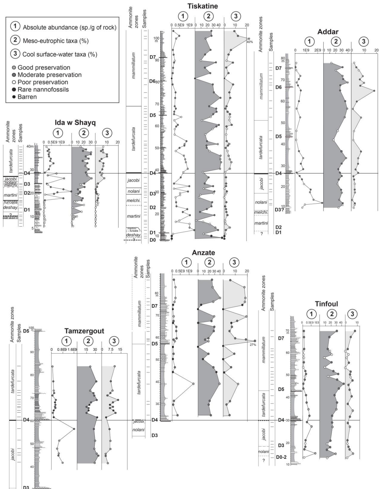
Figure 7. Stratigraphic changes in calcareous nannofossil total absolute abundance and relative abundances of both meso-eutrophic and cold taxa. The sedimentary discontinuities (D0 to D7) are indicated.
