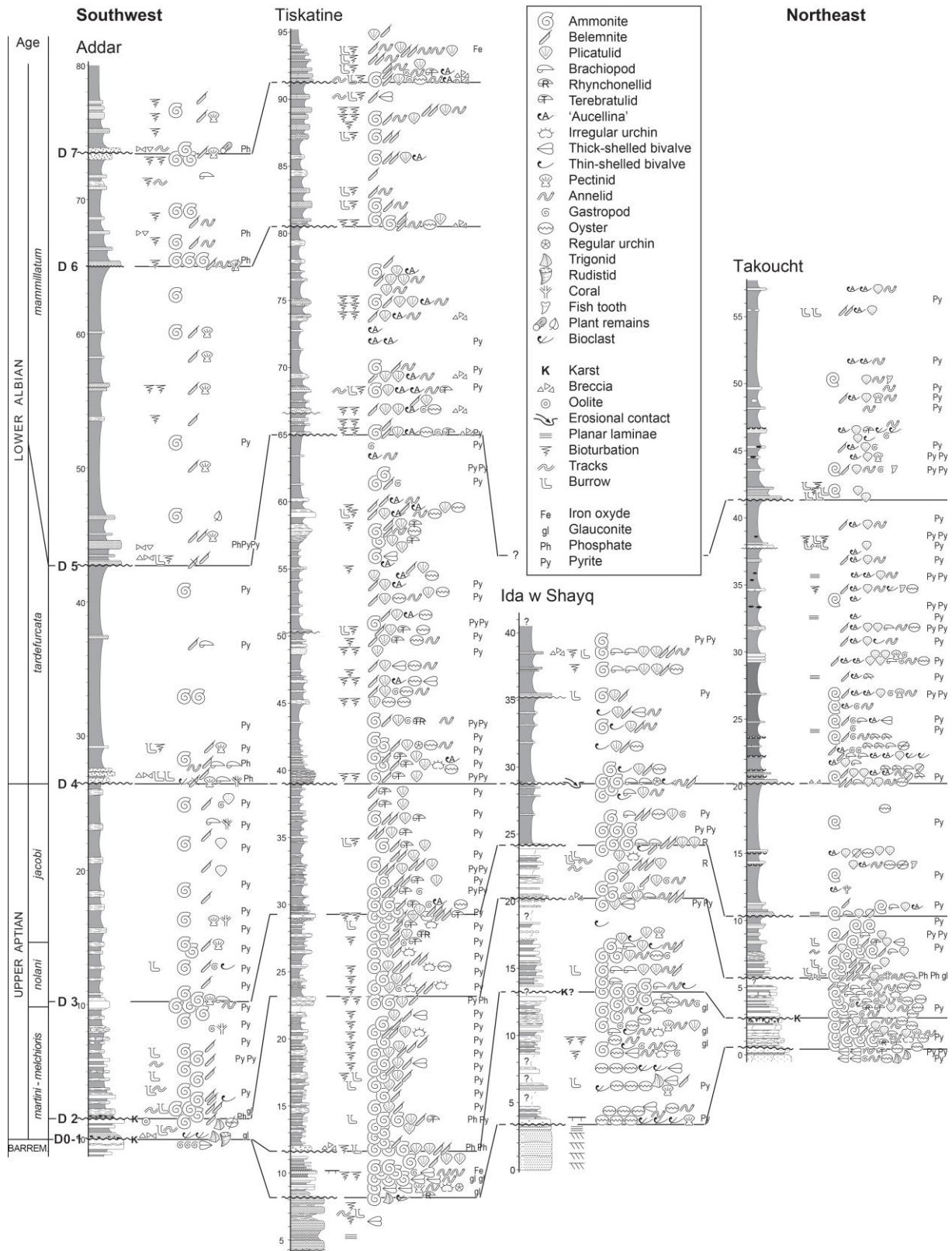
Figure 5. North-South correlations of some Aptian–lower Albian sections of the Essaouira-Agadir basin.
