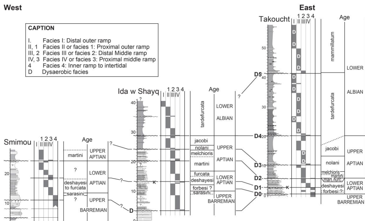
Figure 10. East-West correlations of the Aptian–lower Albian sections in the northern part of the Essaouira-Agadir Basin. D: dysaerobic facies. See Fig. 3 for explanation of 1 to 4, and I to IV.
