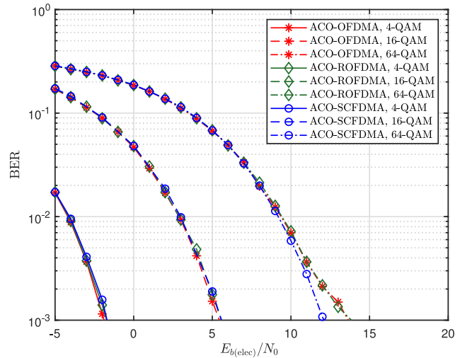
Fig. 12. Contrasting BER performances of ACO schemes for spectral efficiencies of \approx 0.5 bps/Hz (4-QAM), \approx 1 bps/Hz (16-QAM), and \approx 1.5 bps/Hz (64-QAM). P_{t(\text{elec})} = 23 mW. All users placed at D = 3 m from the AP.
