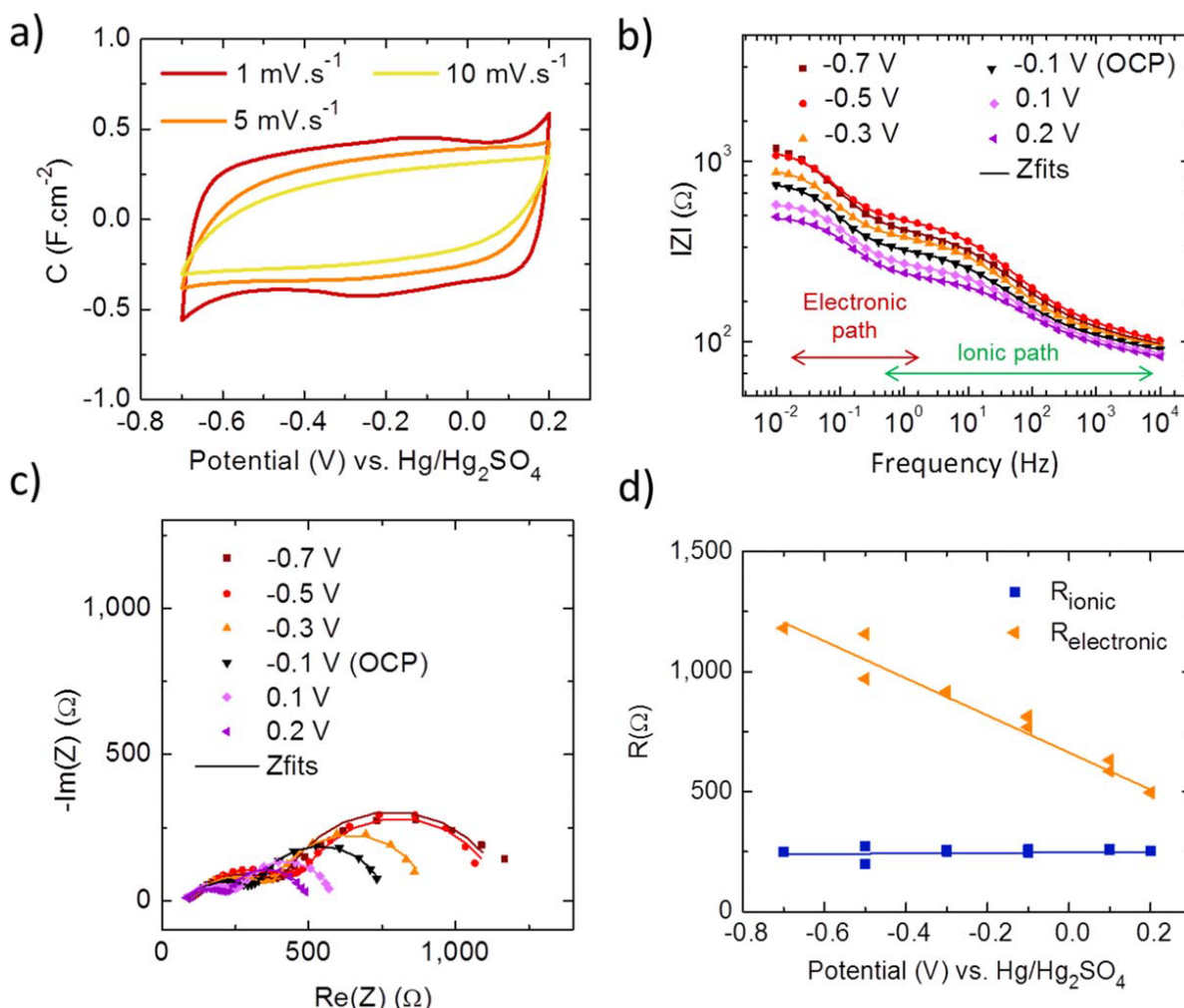
Figure 3. Electrochemical characterization of porous activated carbon. (a) Cyclic voltammetry of a 25 \mu\text{m} thick YP50F electrode in 1 M \text{H}_2\text{SO}_4 vs \text{Hg}/\text{Hg}_2\text{SO}_4 at 1, 5, and 10 \text{mV}\cdot\text{s}^{-1} . (b) Bode plots with corresponding fit lines and (c) Nyquist plots with corresponding fit lines showing the influence that applied voltage has on the activated carbon electrode. (d) Extraction from the total resistance ( R_{\text{TOT}} ) of the ionic ( R_{\text{ionic}} ) and electronic ( R_{\text{electronic}} ) contributions according to the equivalent circuit shown in Fig. 2d.
