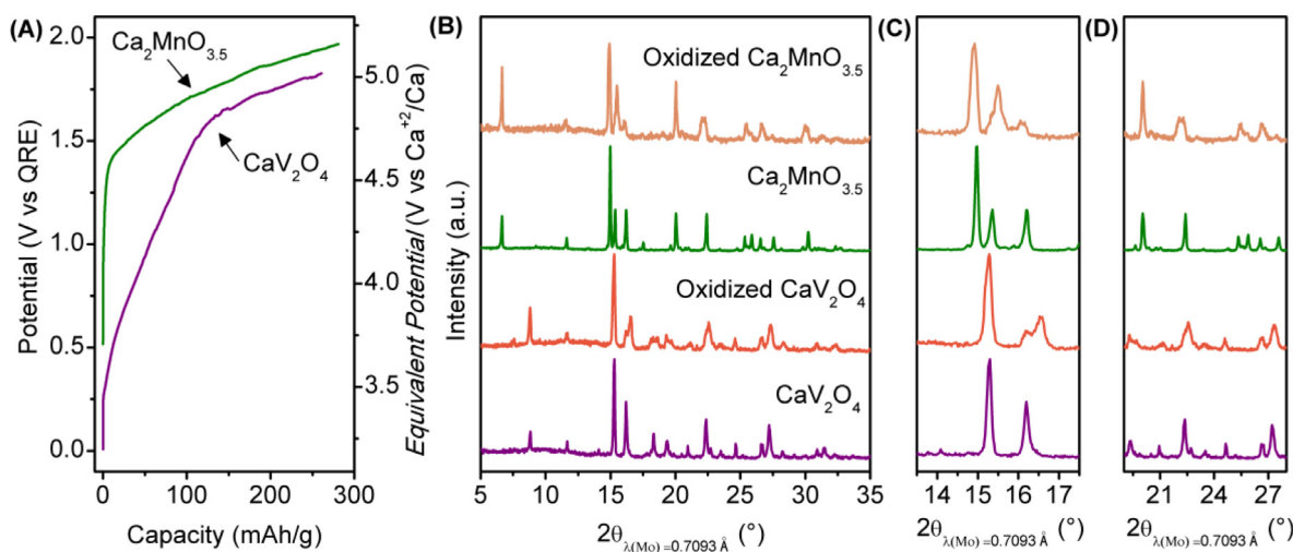
Fig. 3. Voltage vs capacity profiles for \text{CaV}_2\text{O}_4 /AC cells (magenta curve) and \text{Ca}_2\text{MnO}_{3.5} /AC cells (green curve), using 0.45 M \text{Ca}(\text{BF}_4)_2 in EC:PC as electrolyte (A) and corresponding ex situ XRD patterns at the end of oxidation (B). The patterns corresponding to pristine \text{CaV}_2\text{O}_4 and \text{Ca}_2\text{MnO}_{3.5} are also displayed for comparison. Expanded regions of the patterns are depicted in (C) and (D) so that the differences can be more clearly seen.
