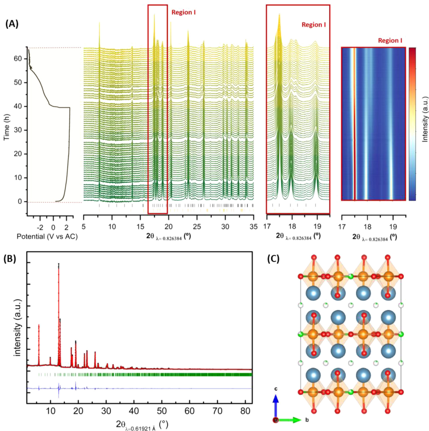
Fig. 4. Characteristic voltage versus time profile for a Ca 2 MnO 3.5 // AC cell using 0.45M Ca(BF 4 ) 2 in EC:PC as electrolyte and corresponding operando synchrotron XRD patterns (A). Calculated and observed XRD patterns for Ca 2 MnO 3.5 electrodes after oxidation in LP30 electrolyte (B). Structural model for Ca 2 MnO 3.5 F 0.6 (C) used for the calculated pattern.
