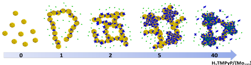
Fig. 5. Schematic representation of hybrid supramolecular aggregates built from Keplerate (yellow), \text{H}_2\text{TMPyP} (blue) and TOS (green). As the \text{H}_2\text{TMPyP} :POM ratio (noted R ) increases, the POM-porphyrin system gives rise to quasi-linear oligomers ( R = 1 ), which then self-arrange into branched-type oligomers ( R = 2 ). For 5 < R < 10 , the hybrid assembly becomes denser giving rise to close-packed aggregates, while for R > 10 , these packed aggregates intercalates tosylate anions strongly immobilized within a porphyrin-based multi-shell around the inorganic capsules.
