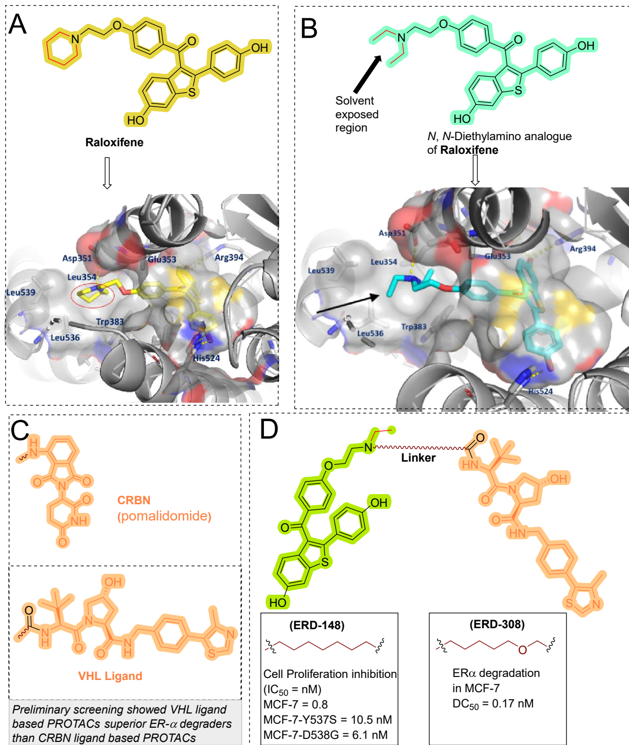
Figure 9. (A) Retrieving the conformational binding of raloxifene with ER- \alpha (PDB 1ERR). (B) Predicted conformational binding of N, N -Diethylamino analogue of Raloxifene with ER- \alpha . (C) Molecular structure of CRBN and VHL ligand. (D) VHL-based PROTACs (ERD-308, ERD-148).
