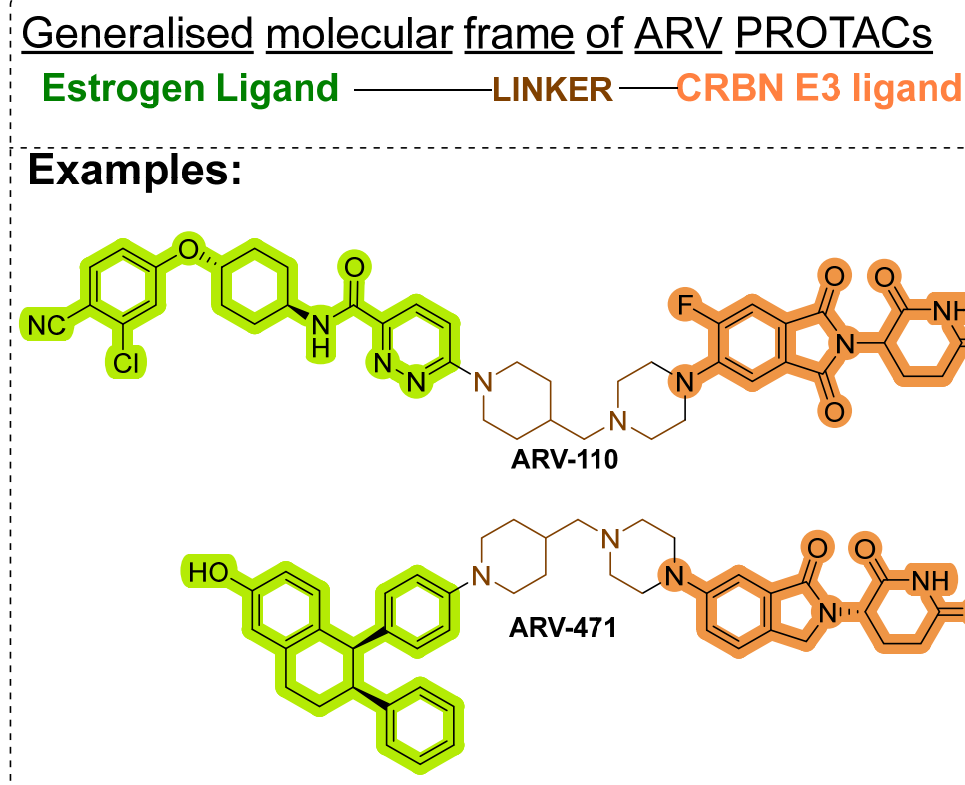
Figure 22. Molecular structure of ARV-110 and ARV-471.
