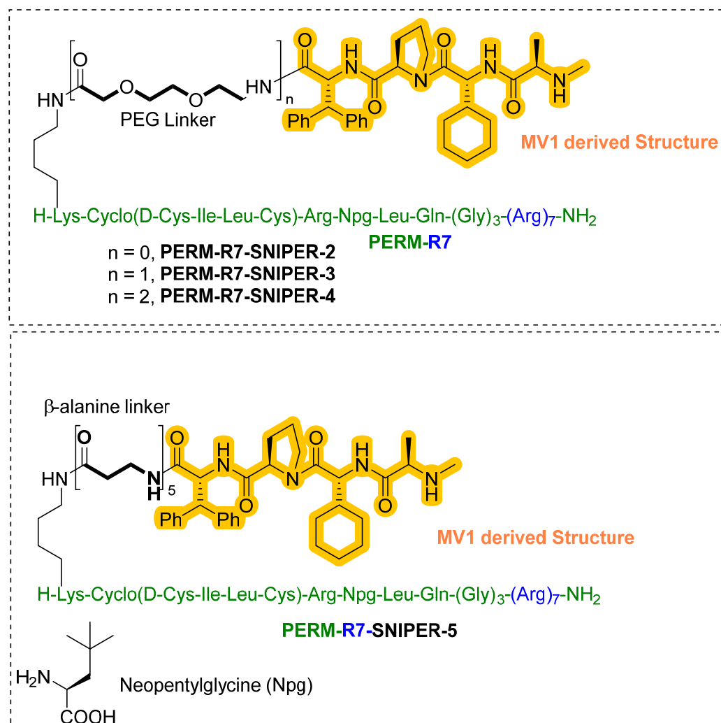
Figure 17. Molecular structure of PERM-R7 (marked in green color) based SNIPERs, which display a hepta-arginine fragment (marked in blue color) and MV1 derived structure (in orange color).
