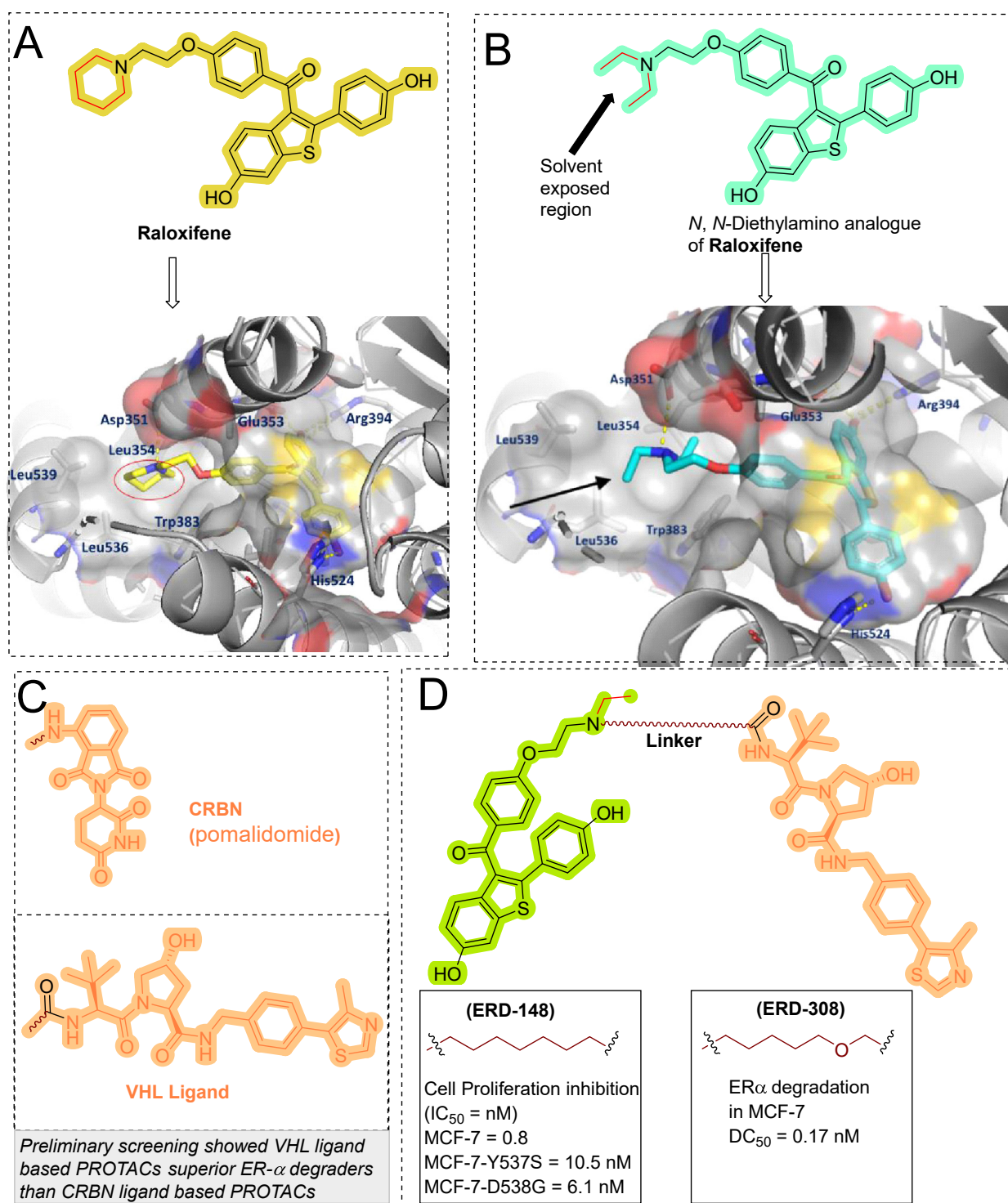
Figure 9. (A) Retrieving the conformational binding of raloxifene with ER- \alpha (PDB 1ERR). (B) Predicted conformational binding of N, N -Diethylamino analogue of Raloxifene with ER- \alpha . (C) Molecular structure of CRBN and VHL ligand. (D) VHL-based PROTACs (ERD-308, ERD-148).
