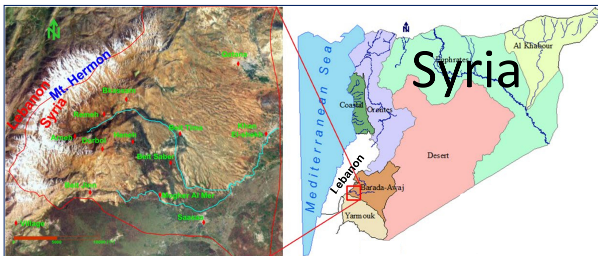
Figure 2. The location of the study area in Barada and Awj Basin (left) and the map of Syria (right), which is divided into seven hydrogeological basins, after the Ministry of Irrigation, Syria, unpublished data.
