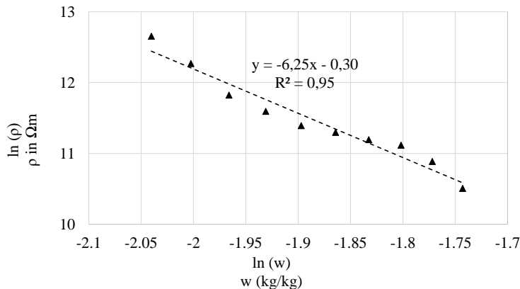
Figure 16: Weighted identification of transition law parameters
