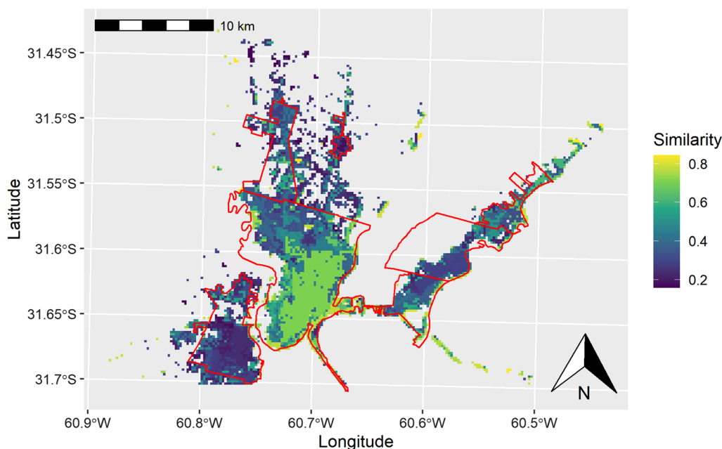
Fig. 3 The Fuzzy Inference System comparison between the environmental and socio-economic suitability for human leptospirosis obtained from both the Conservative and Explorative scenarios
