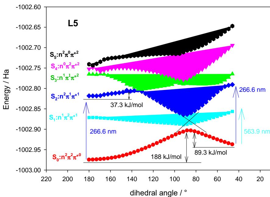
Figure 5 PES scan with respect to -\text{CNNC}- dihedral angle for L5 .
