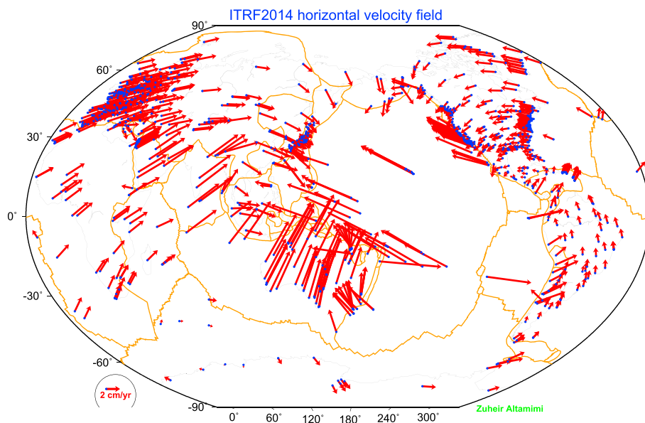
Figure 11. ITRF2014 horizontal site velocities with formal error less than 0.2 mm/yr. Major plate boundaries are shown according to Bird [2003].
