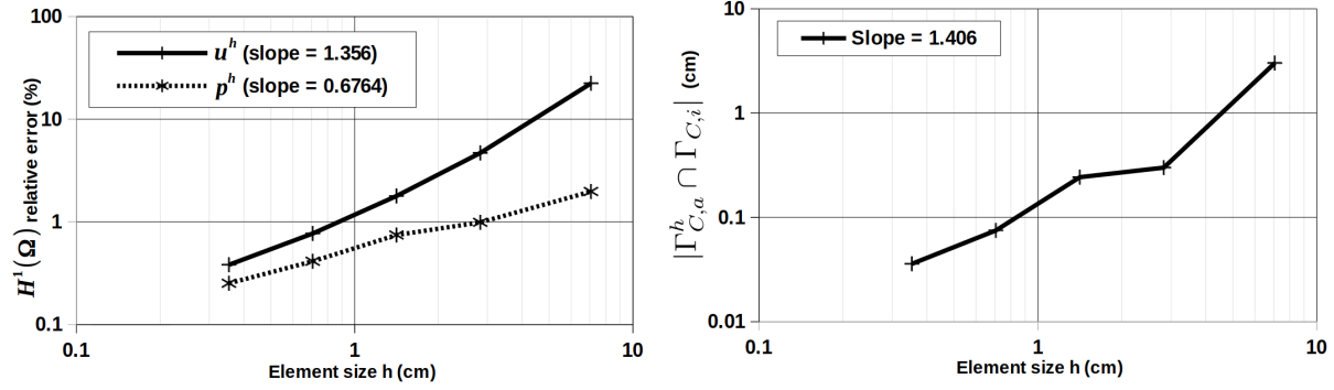
Figure 3: Error curves for \theta = -1 . Left: relative H^1(\Omega) -norm on the displacement and the adjoint state variable. Right: length of \Gamma_{C,a}^h \cap \Gamma_{C,i} .
