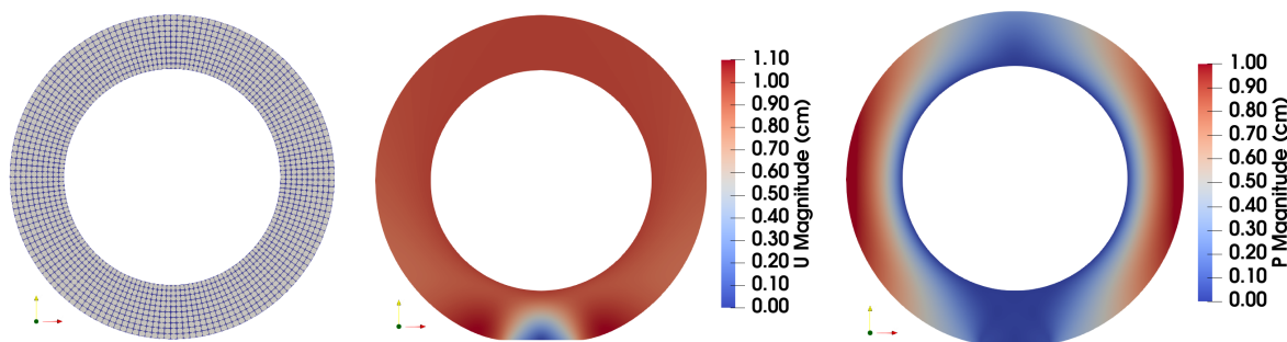
Figure 2: Hollow cylinder in contact with the obstacle. From left to right: structured polar mesh of the hollow cylinder; approximated displacement; approximated adjoint state.
