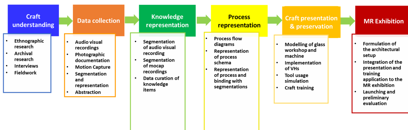
Figure 4. Methodology.
