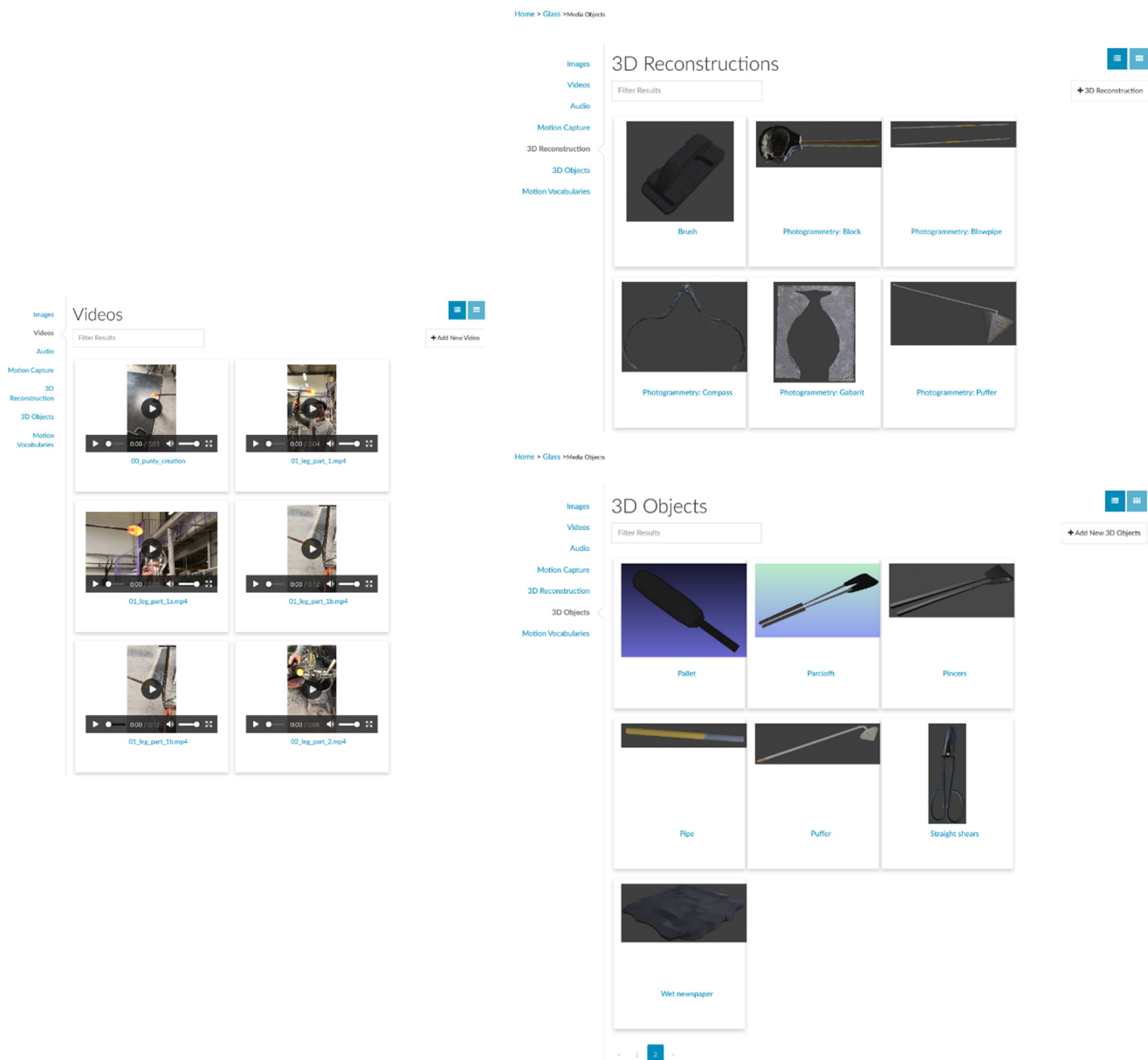
Figure 7. Digital assets.
