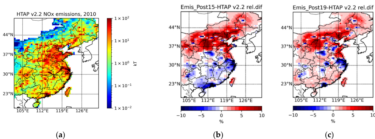
Figure 6. (a) NO x emissions at 0.5° × 0.5° resolution for 2010 from the HTAP v2.2 inventory in kt; Relative differences of NO x emissions for between 2010 and (b) 2015 and (c) 2019, respectively.
