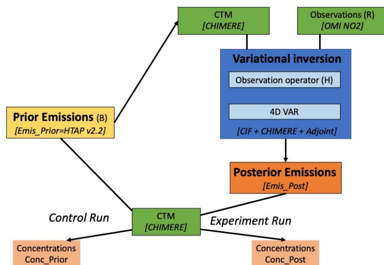
Figure 1. Schematic view of the atmospheric inversion and evaluation in this study.
