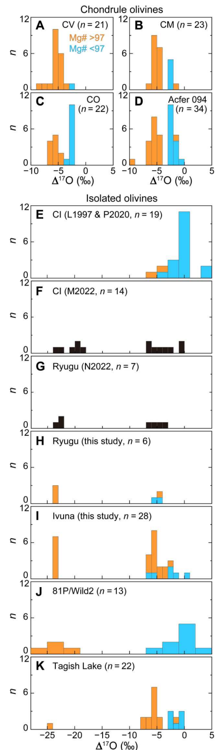
Fig. 1. Histograms of \Delta^{17}\text{O} for olivine grains. Chondrule olivine in (A) CV chondrite Kaba [data from (16)], (B) CM chondrite Murchison [data from (15)], (C) CO chondrite Yamato 81020 [data from (14)], and (D) ungrouped carbonaceous chondrite Acfer 094 [data from (13)]. Isolated olivine grains in (E) CI chondrites Ivuna and Orgueil [previous studies: data from (4, 6)], (F) CI chondrites Ivuna and Alais [previous study: data from (7)], (G) Ryugu [previous study: data from (8)], (H) Ryugu (this study), (I) Ivuna (this study), (J) comet 81P/Wild2 [data from (42, 56–60)], and (K) ungrouped carbonaceous chondrite Tagish Lake [data from (49)]. Magnesium-rich olivine ( \text{Mg}\# > 97 ) is shown as orange and Mg-poor olivine ( \text{Mg}\# < 97 ) in blue, except for (F) and (G) because their chemical compositions are not fully available. Bin sizes of (E) and (J) correspond to their analytical uncertainties. Note that Mg-poor olivine peaks in Yamato 81020 (C) and Acfer 094 (D) may be enhanced because these studies selectively measured Fe-rich ones from the polished sections. The olivine grains with low \Delta^{17}\text{O} are most likely related to refractory inclusions (CAIs and AOAs), while those with high \Delta^{17}\text{O} are related to chondrules. L1997, Leshin et al. (4); P2020, Piralla et al. (6); M2022, Morin et al. (7); N2022, Nakamura et al. (8).
