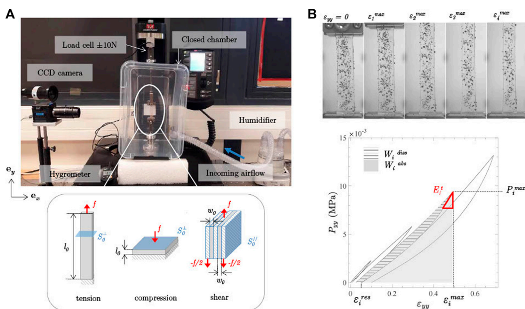
FIGURE 2 (A) Overview of the experimental set-up (top), and schemes illustrating the three loading conditions (tension, compression, shear) applied on the samples (in gray) as well as their dimensions in the reference undeformed configuration (bottom). f represents the average load measured by the load cell. (B) Pictures showing a Ge-GA hydrogel stretched during cyclic tension at increasing peak strain levels, and typical stress-strain response, where the mechanical descriptors introduced to quantify the recorded data for each cycle i ( \epsilon_i^{max} , \epsilon_i^{res} , P_i^{max} , E_i^t , W_i^{diss} , W_i^{abs} ) have been reported.
