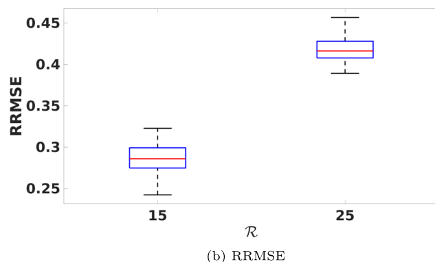
Fig. 9 Box plots of the temperature skill scores: (a) AE and (b) RRMSE for 50 downscaled solutions using DDA with S = 25 and the indicated \mathcal{R}
