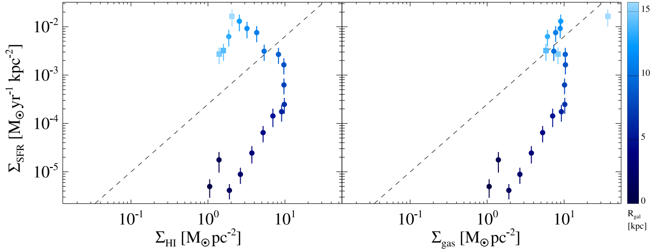
Figure B1. Left: the same as in Figure 7, but with atomic gas surface density on the x -axis (from Nakanishi & Sofue 2016), instead of the molecular one. The KS relation is also plotted as a dashed line. Right: the same as in Figure 7 and in the left panel of this figure, but with total gas surface density on the x -axis. In both panels the x -axis range has been kept identical to that of Figure 7, to facilitate comparison.
