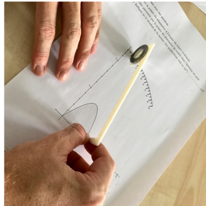
Figure 9: Prytz planimeter
