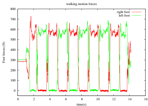
Fig.4 Foot forces during the normal walking
