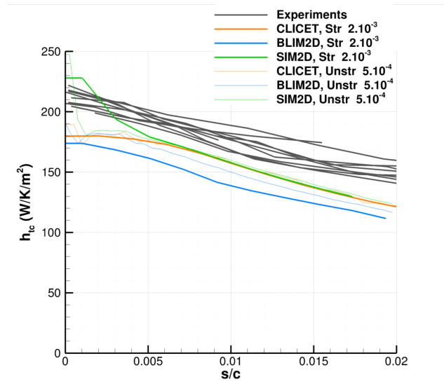
Figure A1. Solution produced by CLICET, SIM2D, and BLIM2D for the heat transfer coefficient with respect to the curvilinear abscissa s in the laminar area of Han and Palacios's experiment for several meshes. Comparison against the experimental measurements.
