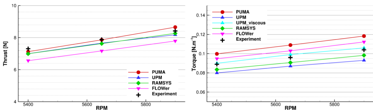
Figure 15: Comparison between experiment and numerical simulations of the KDE12 2 bladed isolated propeller at -10^\circ tilt angle and 12.9 \text{ m.s}^{-1}
