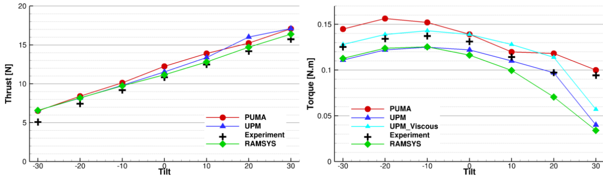
Figure 16: Comparison between experiment and numerical simulations of the KDE12 3 bladed isolated propeller at RPM 5650 and 12.9 \text{ m.s}^{-1}
