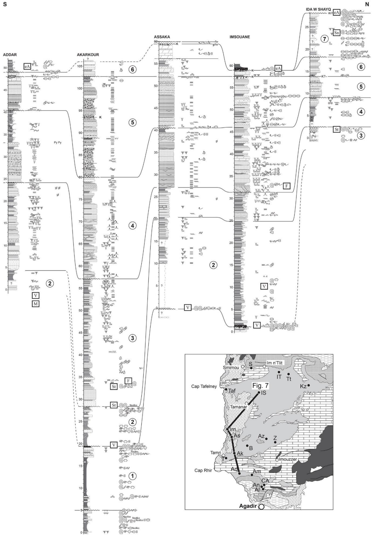
Figure 7. Sedimentary features and N-S correlation of upper Barremian sections in the central and western parts of the study area. Caption of lithologic symbols on Fig. 4. Numbers refer to the units described in the text.
