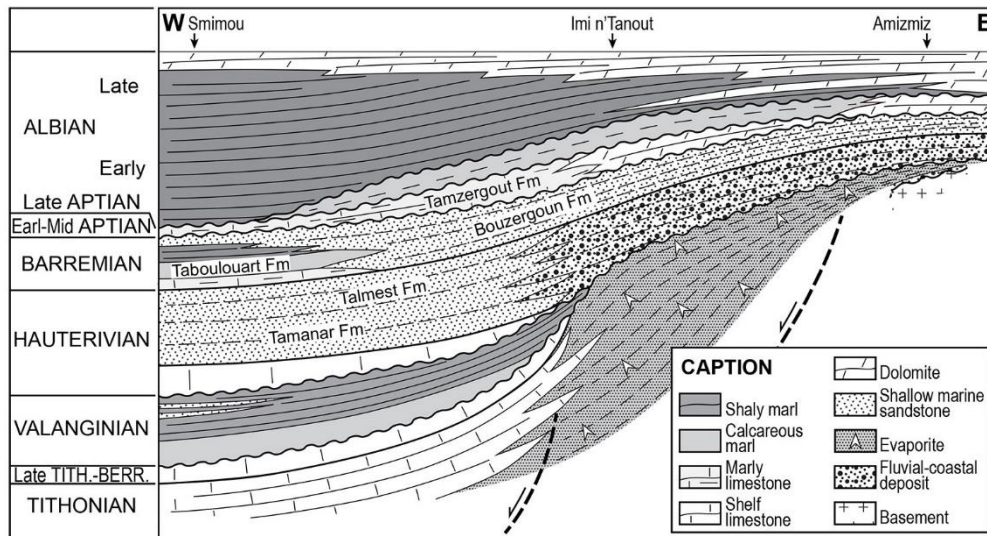
Figure 2. Sketch of the Early Cretaceous sedimentary succession in the northern part of the Essaouira-Agadir Basin, modified from Rey et al. (1988). The maximum thickness of the Cretaceous sequence is about 600 m.
