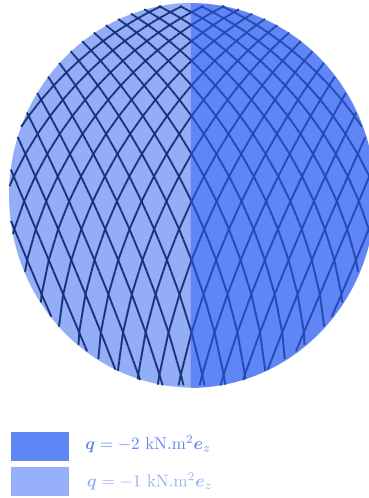
Figure 16: Applied load pattern, seen from top.
