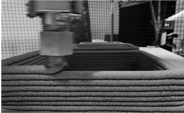
Figure 1: Concrete sample obtained by layer-wise extrusion. Geometrical heterogeneity (layering) is clearly visible, with H = 6\text{mm} , B = 20\text{mm} (Photo: Leo Demont).
