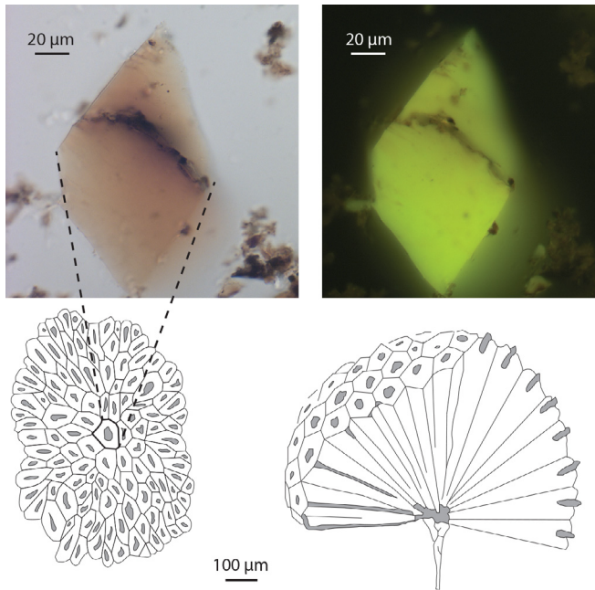
Fig. 7. Views of a Botryococcus Pila colony from above and in a vertical-radial section (after Bertrand and Renault, 1892; Bertrand, 1930 in Alpern, 1981) and one cell of a colony seen in transmitted light and under UV.
