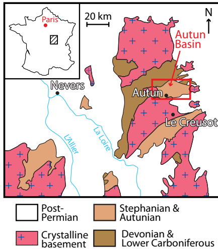
Fig. 1. Location of the Autun Basin in northeastern part of the Massif Central, France (Gand et al. , 2007, modified).
