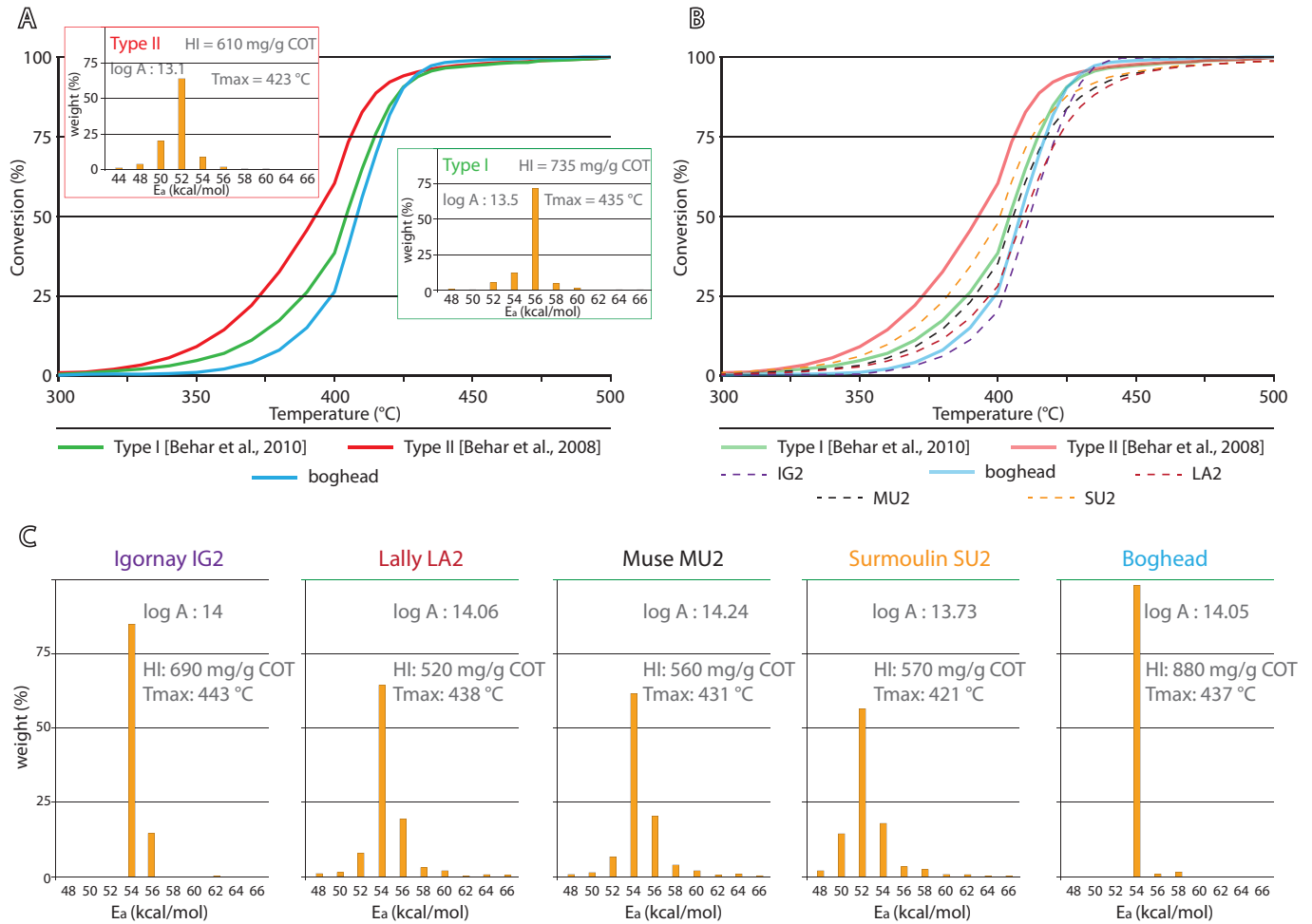
Fig. 6. Conversion curves of kerogens with increasing temperature of: the boghead (this study) and typical Type I from the Green River Shales (Behar et al. , 2010) and Type II from the Toarcian of the Paris Basin (Behar et al. , 2008) kerogens (A); and Autun oil-shales (B). C: kinetic parameters diagrams of the Autun samples (this study).
