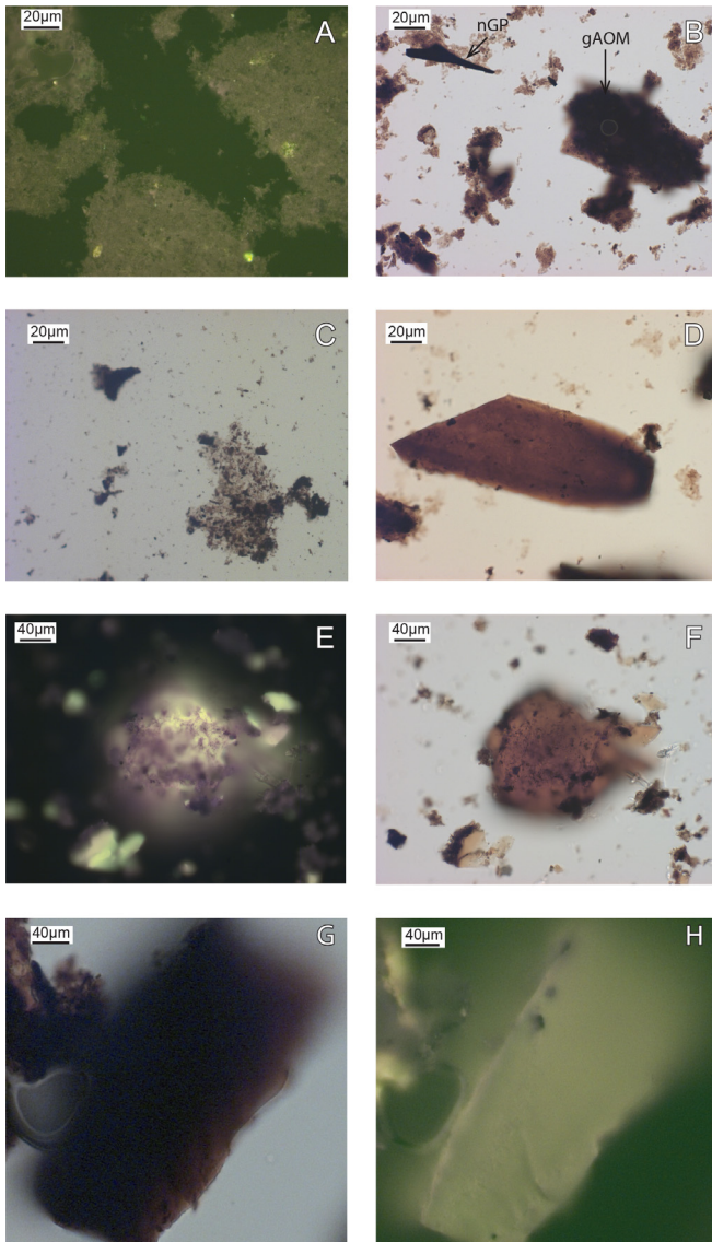
Fig. 4. Palynofacies main categories: (A) fluorescent amorphous organic matter under UV; (B) non-gelified phytoclast (nGP) and gelified amorphous organic matter (gAOM); (C) degraded amorphous organic matter; (D) gelified phytoclast; Botryococcus algae under UV (E) and transmitted light (F); and a gelified cuticle in transmitted light (G) and under UV (H).
