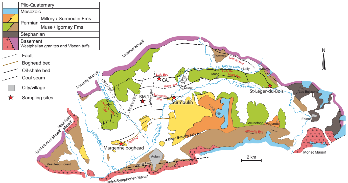
Fig. 2. Simplified geological map of the Autun Basin and location of sampling sites (Gand et al. , 2007, modified).
