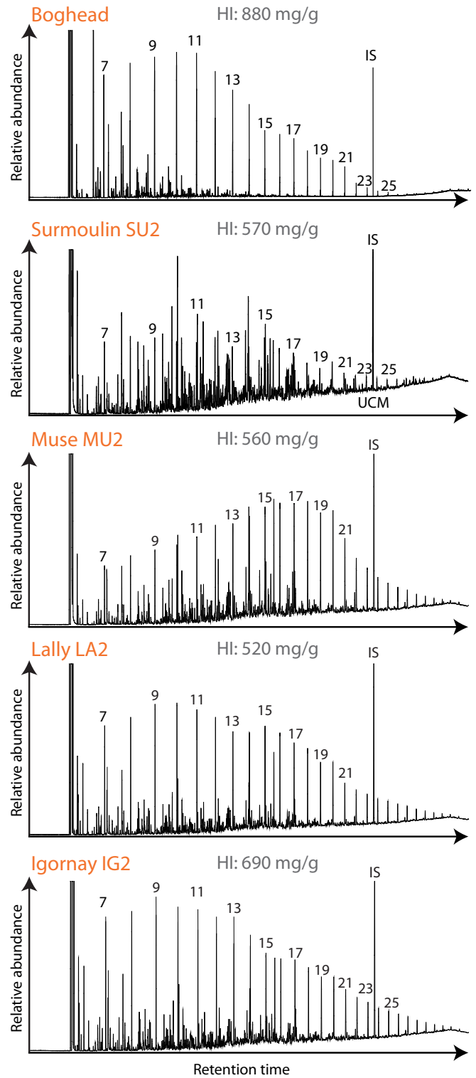
Fig. 5. GC-FID of hydrocarbons obtained during closed system pyrolysis of the boghead, Surmoulin SU2, Muse MU2, Lally LA2, and Igornay IG2 samples, representative of the groups defined in the results section. Numbers above peaks represent carbon number of the respective n -alkane. IS = internal standard; UCM: unresolved complex mixture.
