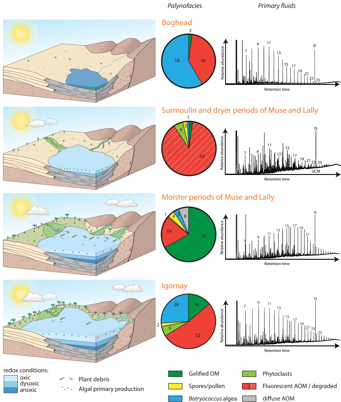
Fig. 8. Palaeogeographic sketch of the Autun lake evolution during oil-shale and boghead deposition compared with OM content and HC distribution. IS = internal standard; UCM: unresolved complex mixture.
