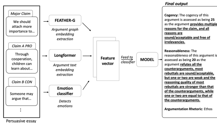
Figure 2. Overview of our natural language argumentation quality prediction model.
