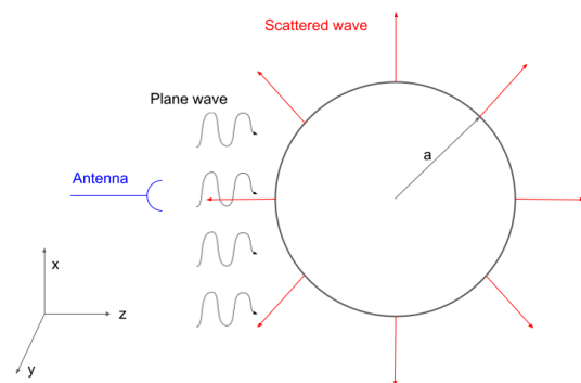
Figure 1: Setting of the scattering by a sphere.
