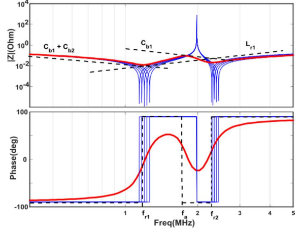
Fig. 8. Measured impedance (red), model (blue): variation of L_1 to \pm 20\% at the turn of the measurement, asymptotic trend (black dotted line).
