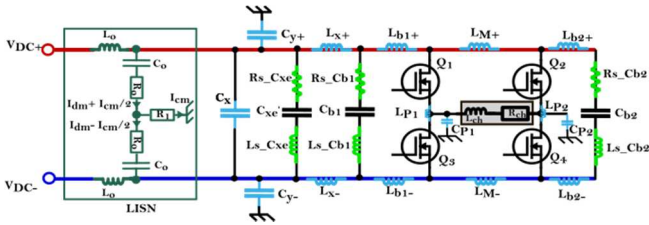
Fig. 9 Complete power model with an upstream LISN ( R_0 = 27 \Omega , R_1 = 39 \Omega , C_0 = 220 \text{ nF} and L_0 = 250 \mu\text{H} )
