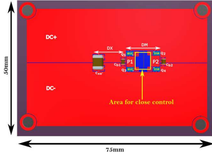
Fig. 3. Full Bridge converter top side routing
