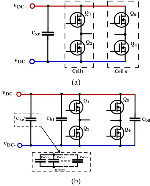
Fig. 1. Scheme of a complete bridge chopper with its decoupling capacitor
