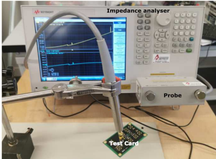
Fig. 4. Photograph of the measuring bench
