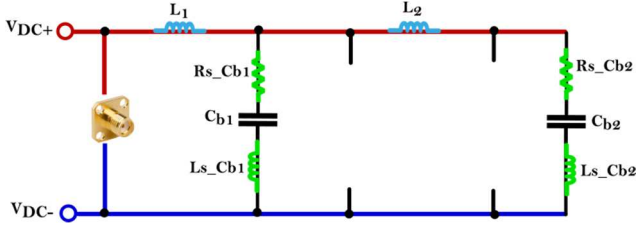
Fig. 6. Equivalent diagram for the measurement of the parasitic inductances of the power tracks
