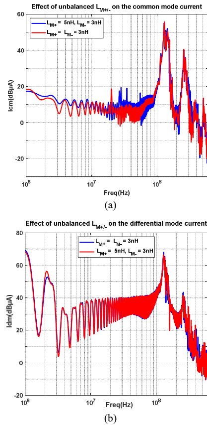
Fig. 11. Effect of L_{M+/-} unbalance on common mode (a) and differential mode (b) current
