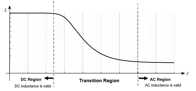
Fig. 5. Inductance of a conductor as a function of frequency [10]
