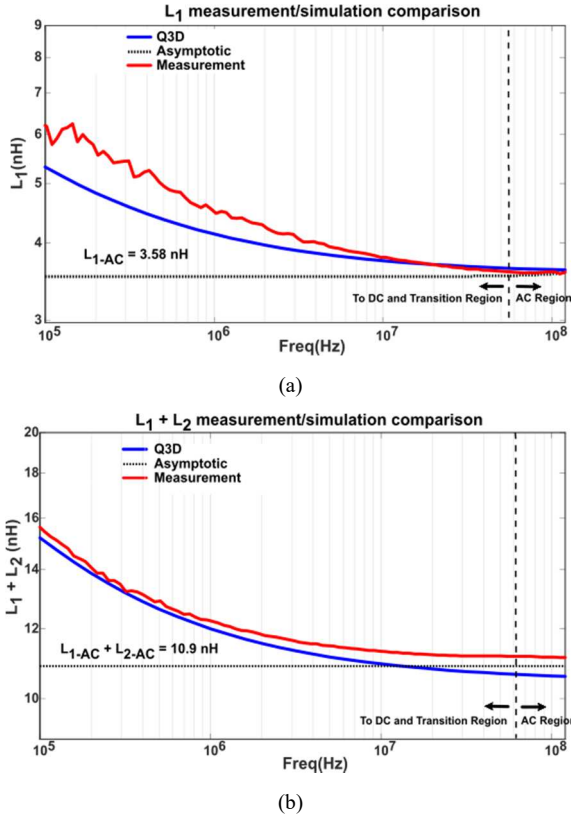
Fig. 7 L_1 inductance measurement (red) compared to the simulation (blue) and to the asymptotic value (black dotted line): L_1 (a) and L_1 + L_2 (b)
