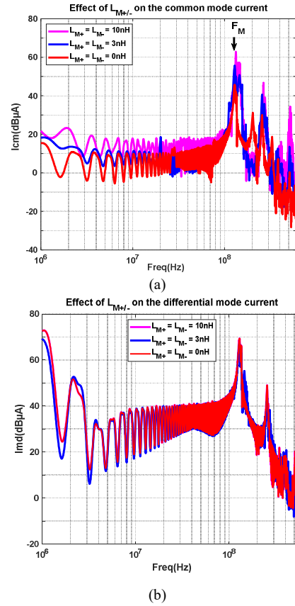
Fig. 10. Common (a) and differential (b) mode current as a function of L_{M+/-}
