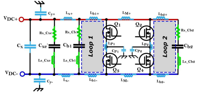
Fig. 2. Diagram of the EMC equivalent model on the power side
