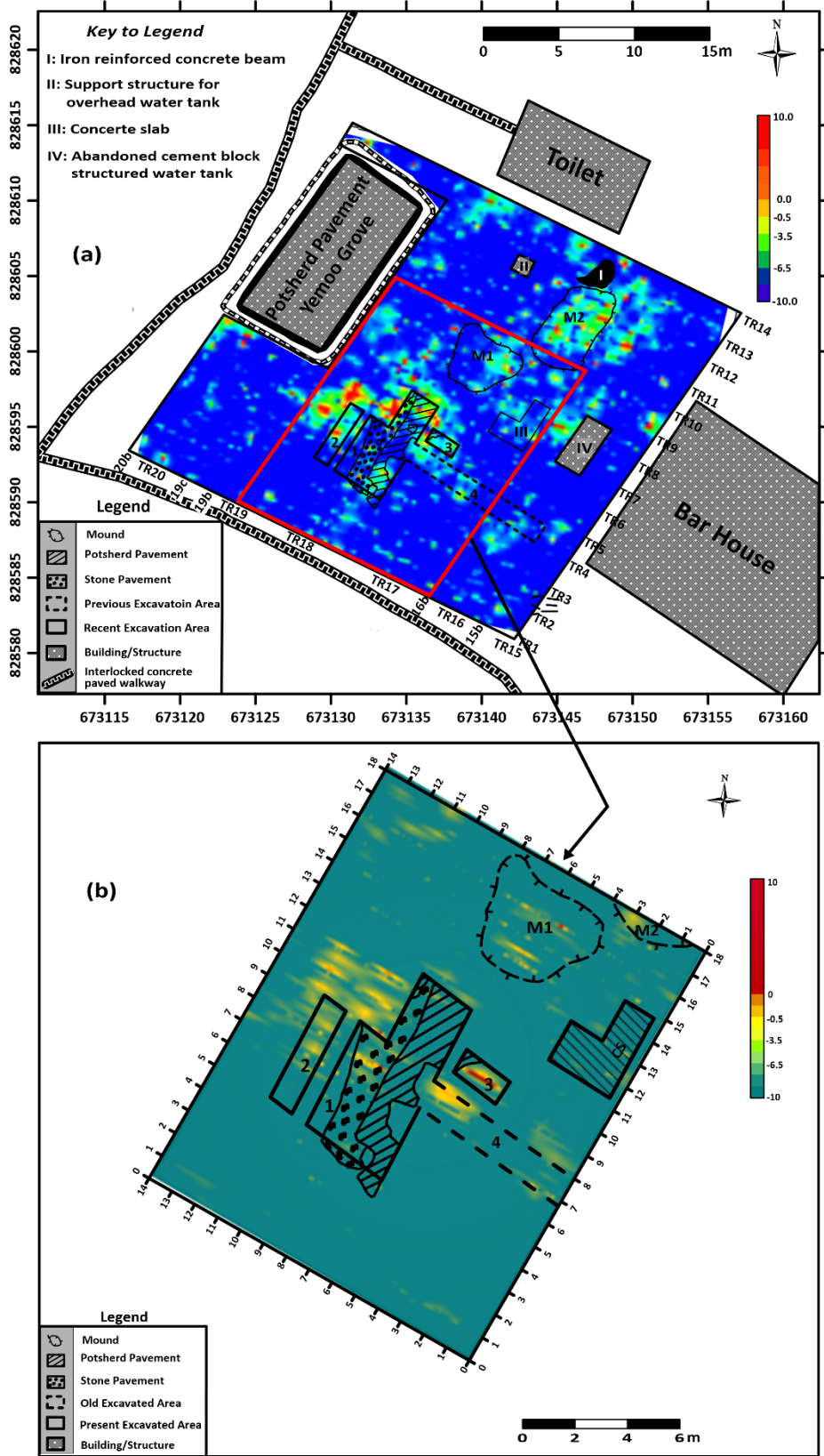
Fig. 31(a): 2D GPR depth slice map at 0.75 m and (b) 3D GPR depth slice map at 0.75 m
