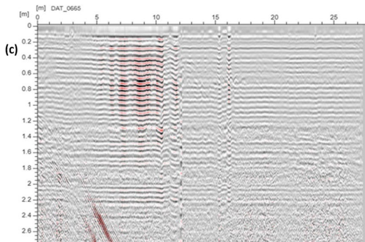
Fig. 26: (b) Vertical section radargram (450 MHz) along Traverse TR5 and (c) Vertical section radargram (750 MHz) along Traverse TR5
