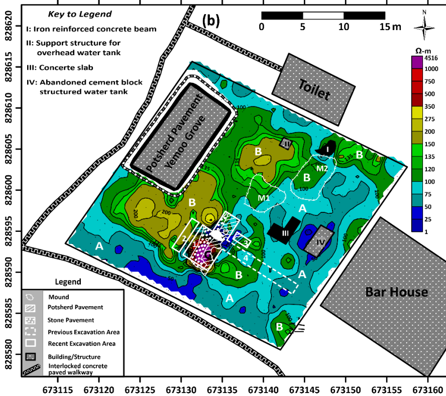
Fig. 17: Apparent resistivity maps at (a) expansion factor ( n ) of 1 and theoretical depth of 0.59 m and (b) expansion factor ( n ) of 2 and theoretical depth of 0.78 m
