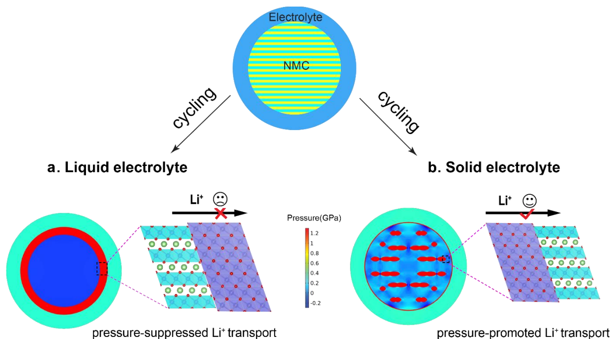
Fig. 4. Stress-mediated \text{Li}^+ transport kinetics in liquid and solid electrolytes. (a) In liquid electrolytes, electrochemical cycling forms a thick RSP ( \sim 20\text{-}200 nm) at the NMC/electrolyte interface. The lattice mismatch between the phases generates compression in the RSPs (red) and tension in the layered structures (blue). The dense, highly compressed RSPs function as an impermeable layer that traps all the remaining \text{Li}^+ in the interior layered phases, causing considerable capacity loss. (b) In solid electrolytes, electrochemical cycling forms RSPs that are dispersed into the bulk of the NMC particle. The compressive stress in the RSPs (red) squeezes \text{Li}^+ out of the RSPs into the adjacent layered phases (light blue/blue), and the layered phases form a percolation channel that conducts \text{Li}^+ further out of the NMC particle, rendering an electrochemically active RSPs.
